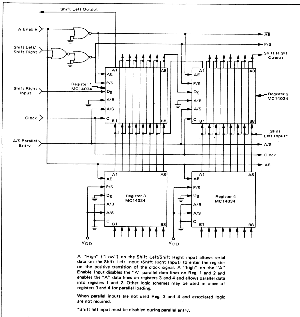
FIGURE 6 – SHIFT RIGHT/SHIFT LEFT WITH PARALLEL INPUTS
