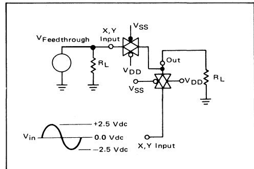
FIGURE 10 – FREQUENCY RESPONSE TEST CIRCUIT
