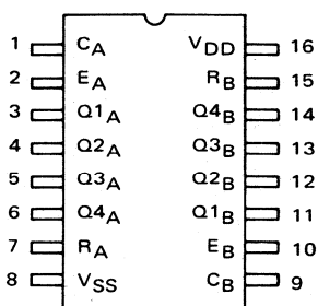
MC14518 Dual BCD Up Counter
