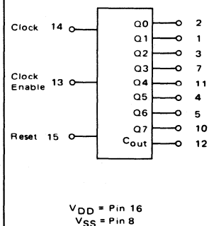
MC14022 Octal Counter/Divider
