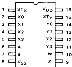
MC14529 Dual 4-Channel Analog Data Selector
