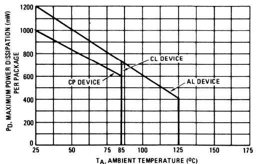
FIGURE 1 – AMBIENT TEMPERATURE POWER DERATING
