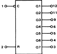
MC14024 Seven-Stage Ripple Counter
