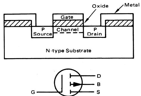
FIGURE 1-1 — P-CHANNEL TRANSISTOR (PMOS)
