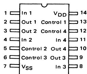
MC14016 Quad Analog Switch/Quad Multiplexer
