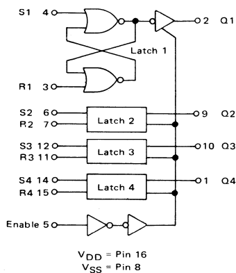
MC14043 Quad NOR R-S Latch (Three-State Outputs)
