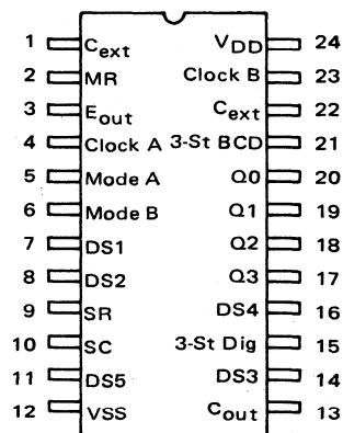
MC14534 Real Time 5-Decade Counter
