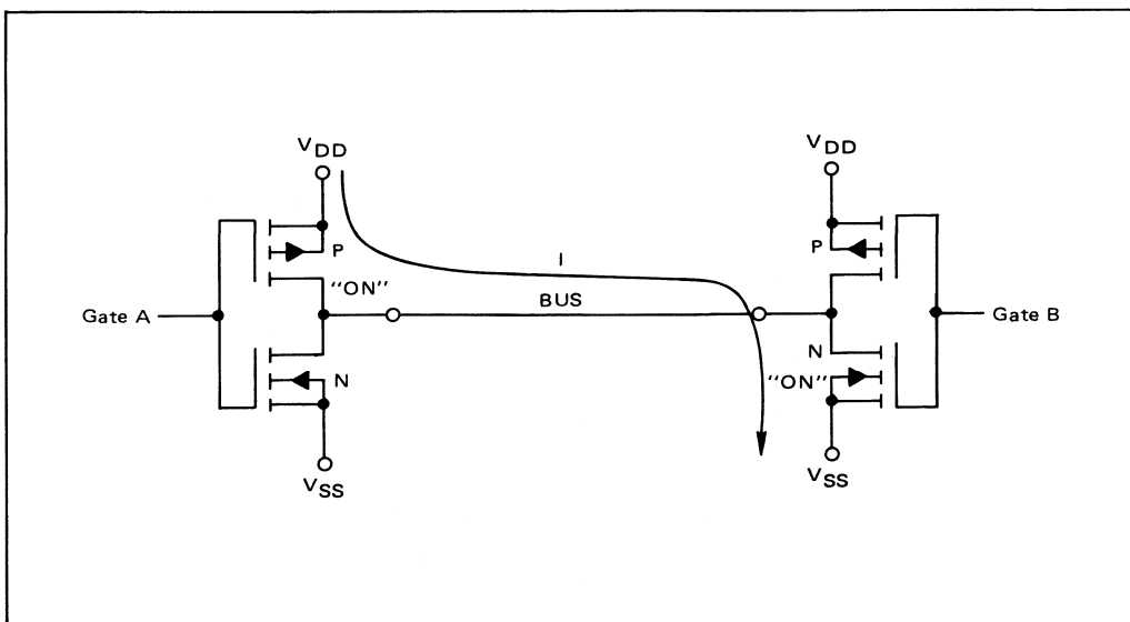
FIGURE 2-31 – CMOS GATES WITH OUTPUTS CONNECTED
