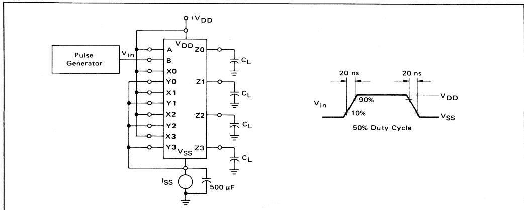
FIGURE 1 – DYNAMIC POWER DISSIPATION TEST CIRCUIT AND WAVEFORM
