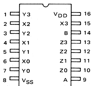
MC14519 4-Bit AND/OR Selector
