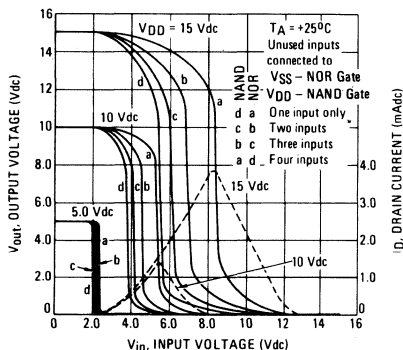
FIGURE 1 – VOLTAGE AND CURRENT TRANSFER CHARACTERISTICS (4-Input Gate)
