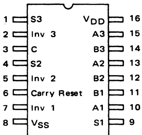
MC14038 Triple Serial Adder (Negative Logic)
