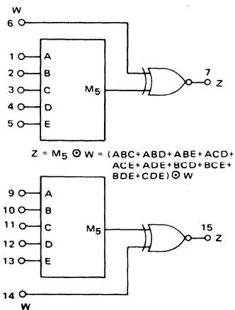
MC14530 Dual 5-Input Majority Logic Gate
