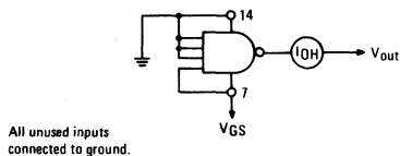
FIGURE 1 – TYPICAL OUTPUT SOURCE CHARACTERISTICS TEST CIRCUIT
