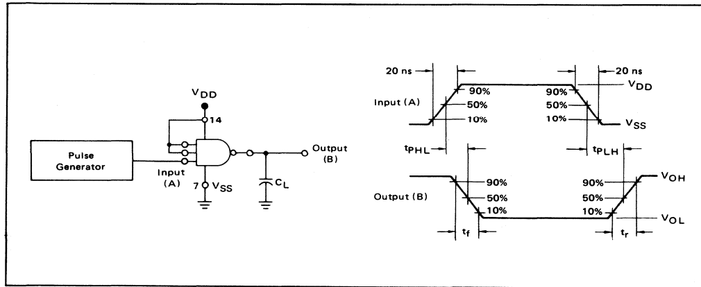
FIGURE 4 – SWITCHING TIME TEST CIRCUIT AND WAVEFORM
