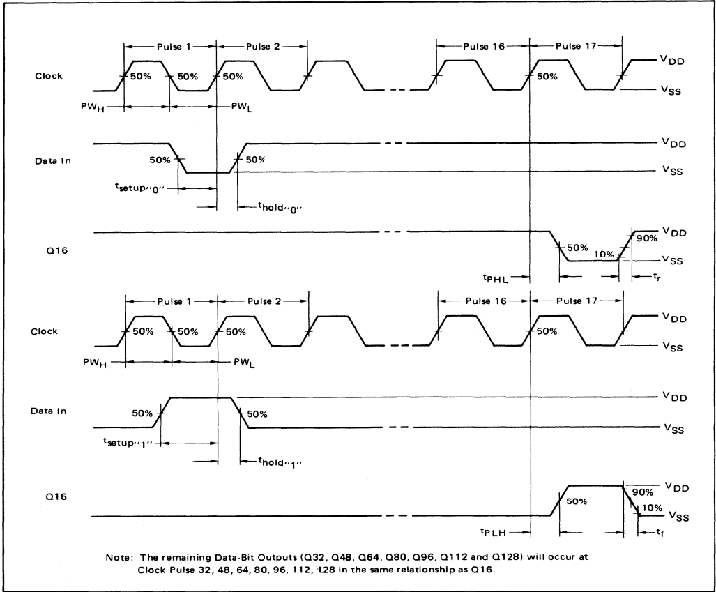
AC TEST WAVEFORMS
