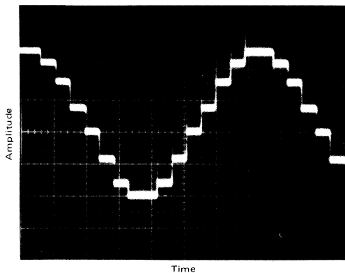
FIGURE 1 – TYPICAL SINE WAVE OUTPUT (Pins 2 or 15, No External Filtering)
