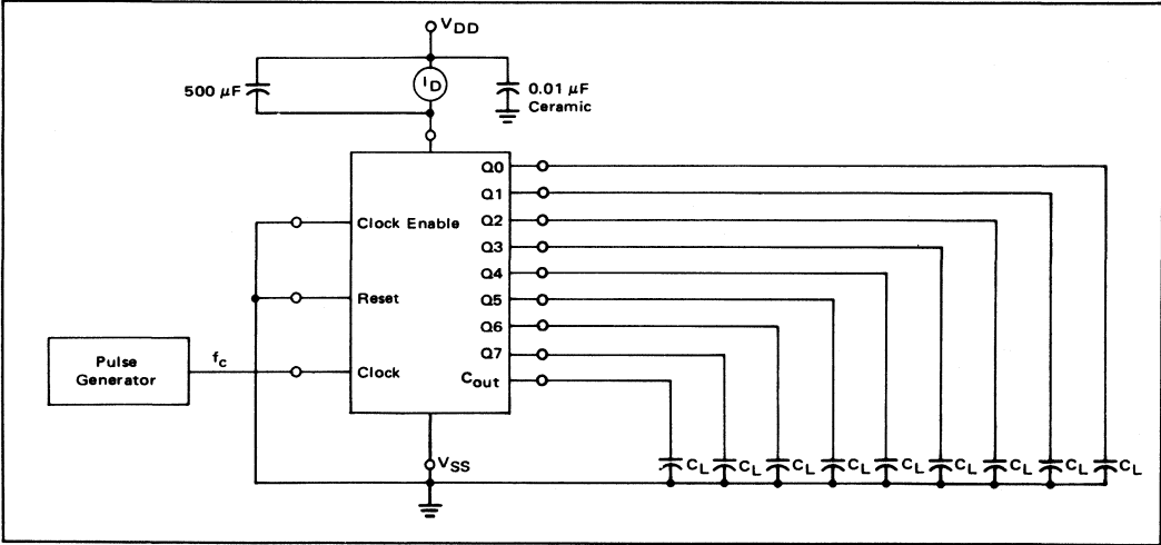
FIGURE 2 – TYPICAL POWER DISSIPATION TEST CIRCUIT
