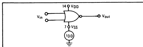
FIGURE 1 – CURRENT AND VOLTAGE TRANSFER CHARACTERISTICS TEST CIRCUIT
