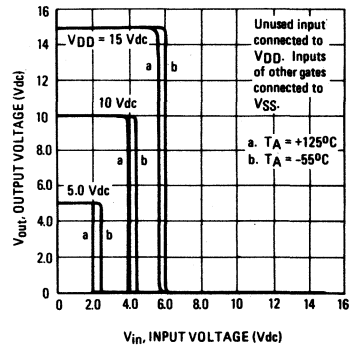
FIGURE 3 – TYPICAL VOLTAGE TRANSFER CHARACTERISTICS versus TEMPERATURE
