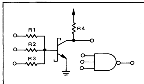
FIGURE 2-25 — A BASIC STRL GATE
