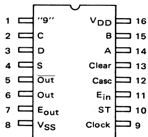
MC14527 BCD Rate Multiplier
