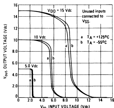
FIGURE 2 – VOLTAGE TRANSFER CHARACTERISTICS versus TEMPERATURE
