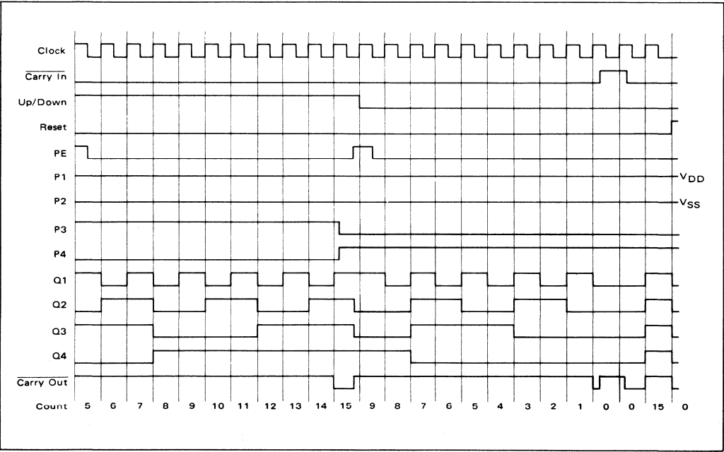
TIMING DIAGRAM
