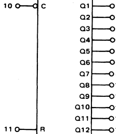
MC14040 12-Bit Binary Counter
