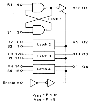
MC14044 Quad NAND R-S Latch (Three-State Outputs)
