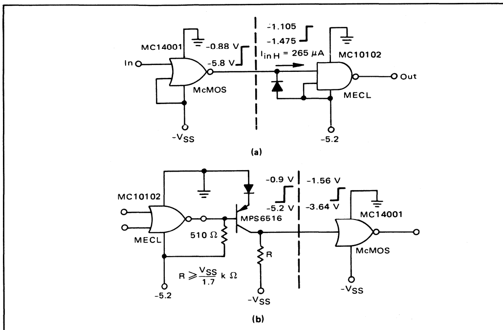
FIGURE 2-23 -McMos-MECL AND MECL-McMos INTERFACE SYSTEMS
