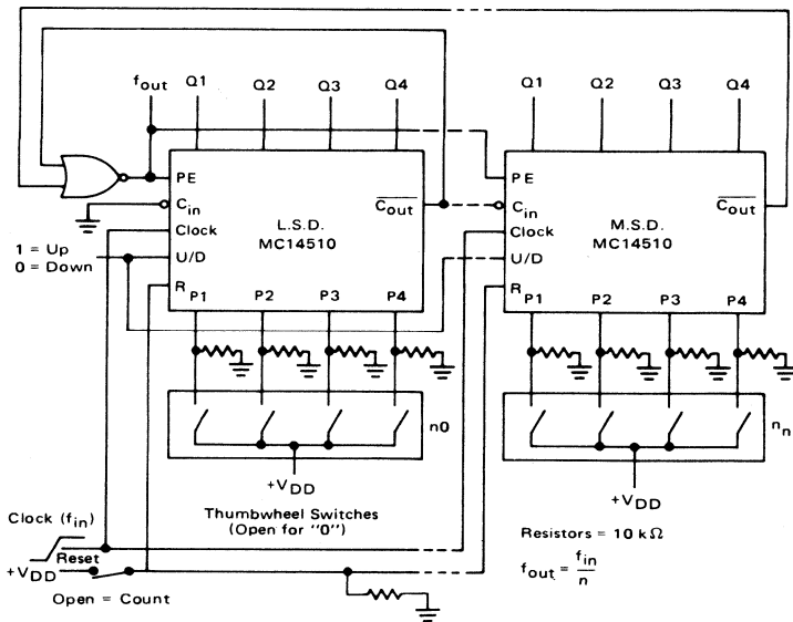
FIGURE 4 – PROGRAMMABLE CASCADED FREQUENCY DIVIDER
