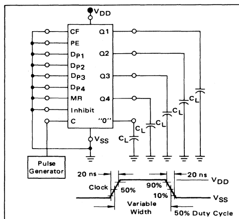
FIGURE 3 – POWER DISSIPATION
