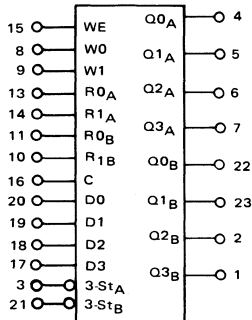
MC14580 4 x 4 Multiport Register
