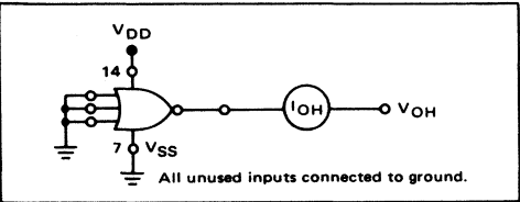
FIGURE 4 – TYPICAL OUTPUT SOURCE CHARACTERISTICS TEST CIRCUIT
