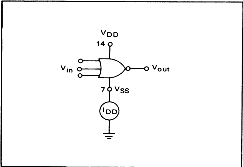
FIGURE 1 – CURRENT AND VOLTAGE TRANSFER CHARACTERISTICS TEST CIRCUIT
