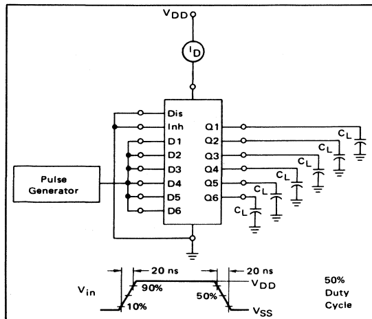
FIGURE 3 — POWER DISSIPATION TEST CIRCUIT AND WAVEFORM
