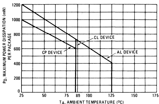
FIGURE 4 — AMBIENT TEMPERATURE POWER DERATING
