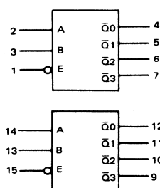
MC14556 Dual Binary To 1-of-4 Decoder/Demultiplexer
