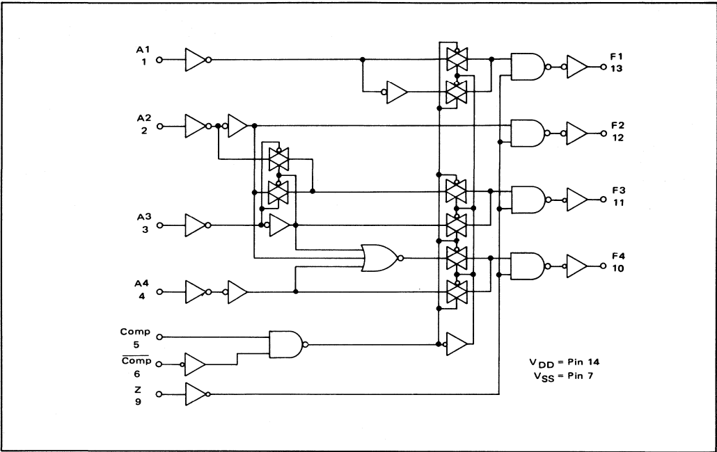
LOGIC DIAGRAM
