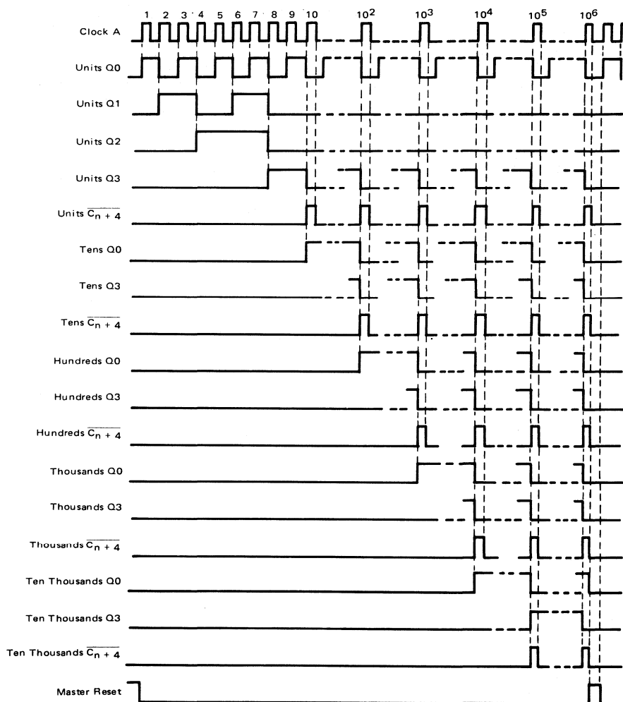
COUNTER TIMING DIAGRAM
