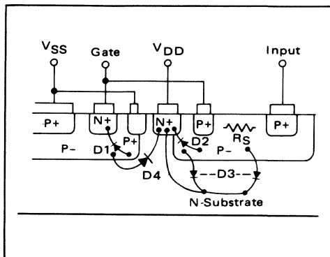
FIGURE 2-13(a) - PHYSICAL DIAGRAM, DIODE-RESISTOR INPUT PROTECTION
