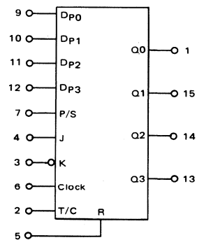
MC14035 4-Bit Parallel In/Parallel Out Shift Register
