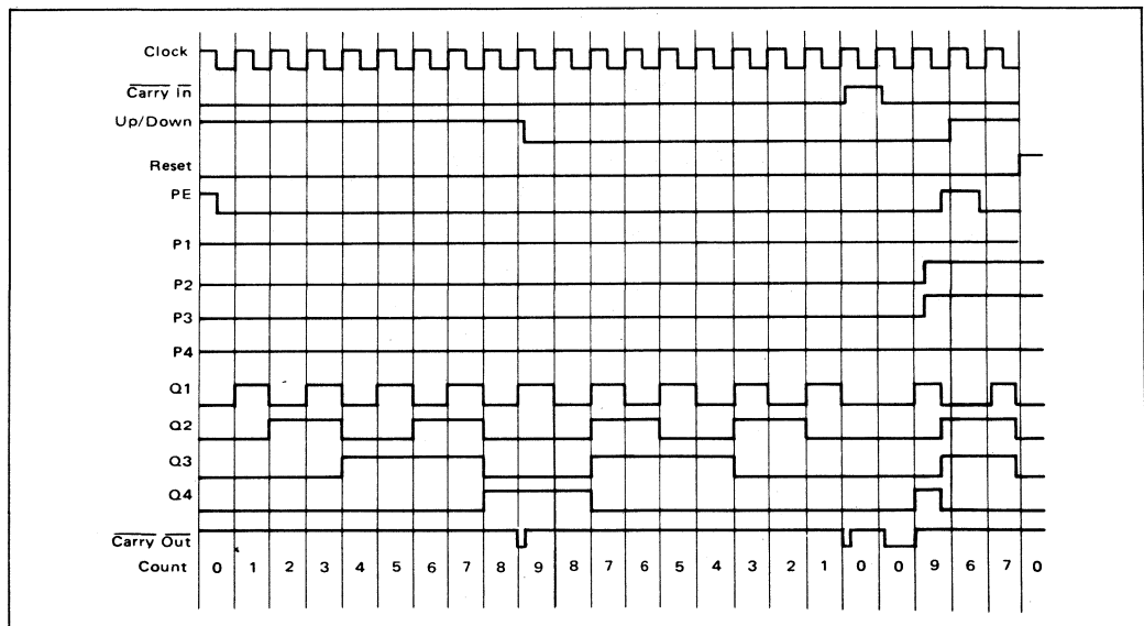
TIMING DIAGRAM
