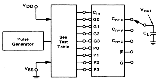
FIGURE 4 – SWITCHING TIME TEST CIRCUIT AND WAVEFORMS
