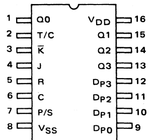
MC14035 4-Bit Parallel-In/Parallel Out Shift Register
