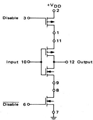
FIGURE 5 – 3-STATE BUFFER
