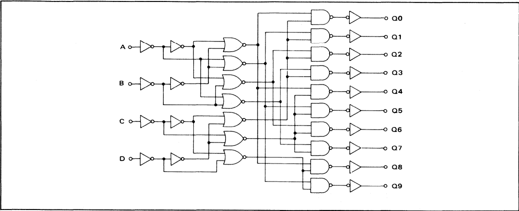
LOGIC DIAGRAM
