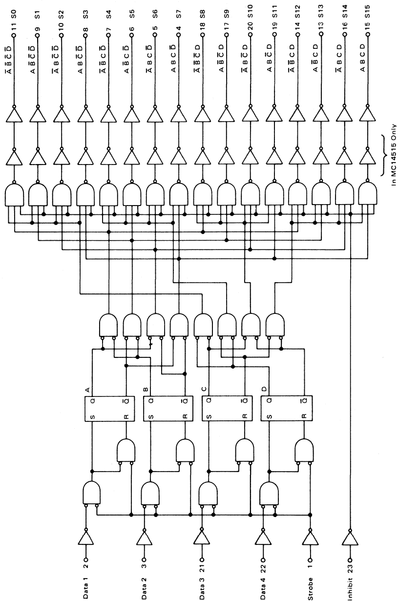
LOGIC DIAGRAM
