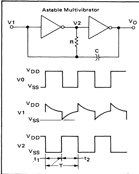
FIGURE 2-14 – ASTABLE MULTIVIBRATOR
