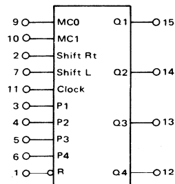
MC14194 4-Bit Bidirectional Universal Shift Register
