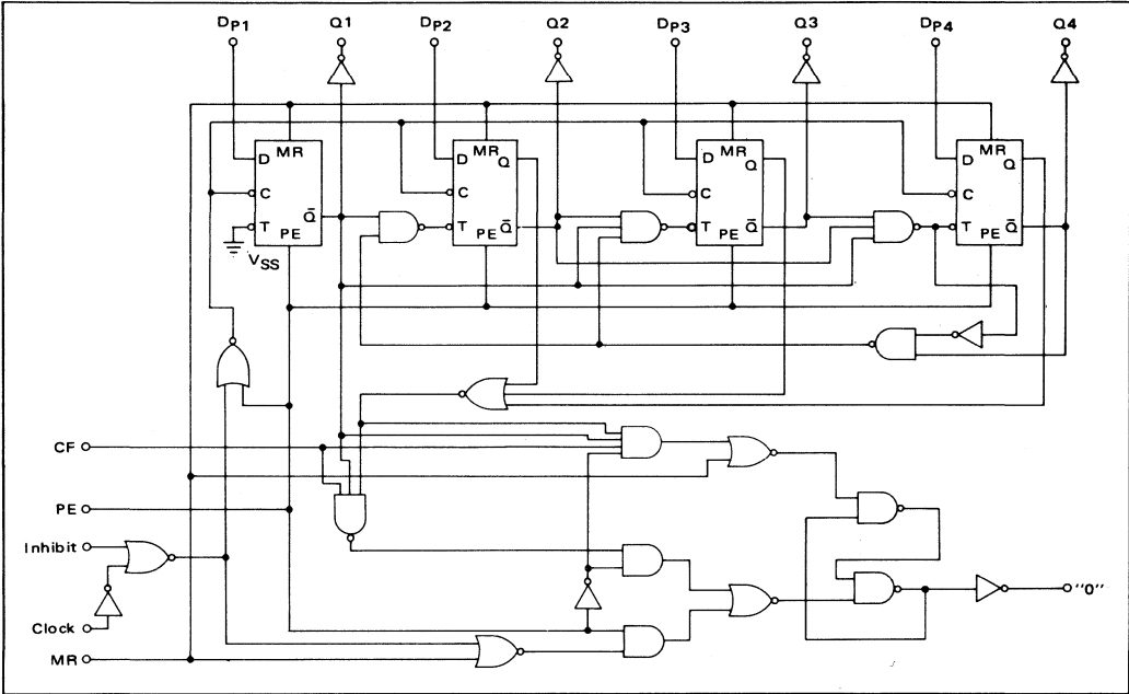
FIGURE 7 – MC14526 LOGIC DIAGRAM (Binary Divide-by-N Counter)
