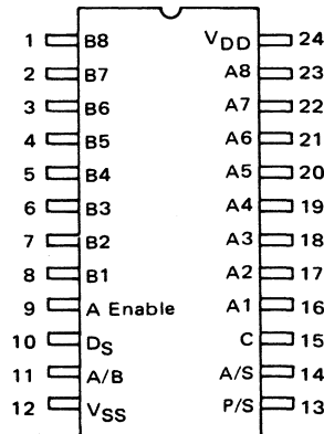
MC14034 8-Bit Universal Bus Register
