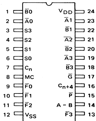
MC14581 4-Bit Arithmetic Logic Unit
