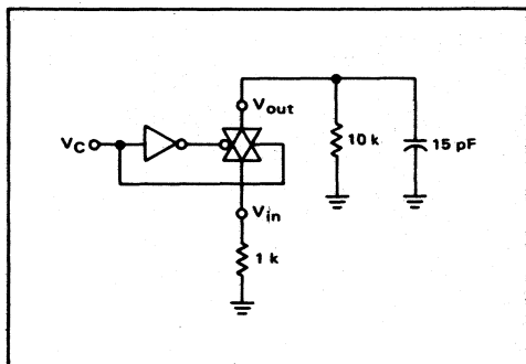
FIGURE 10 – CROSSTALK TEST CIRCUIT
