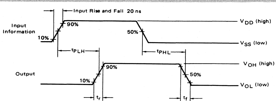
FIGURE 5-14 – NON-SYNCHRONOUS CIRCUIT WAVESHAPES AND TIMING PARAMETERS
