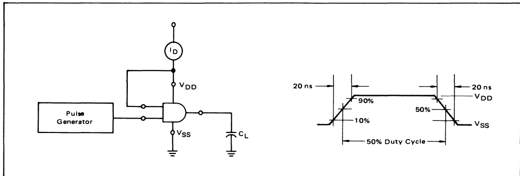
FIGURE 4 – POWER DISSIPATION TEST CIRCUIT AND WAVEFORM
