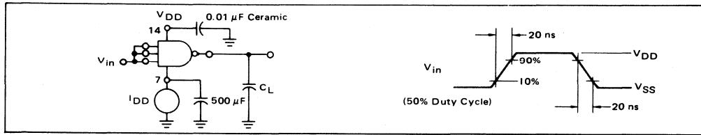
FIGURE 3 – POWER DISSIPATION TEST CIRCUIT AND WAVEFORM
