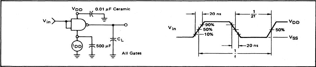
FIGURE 3 – POWER DISSIPATION TEST CIRCUIT AND WAVEFORM
