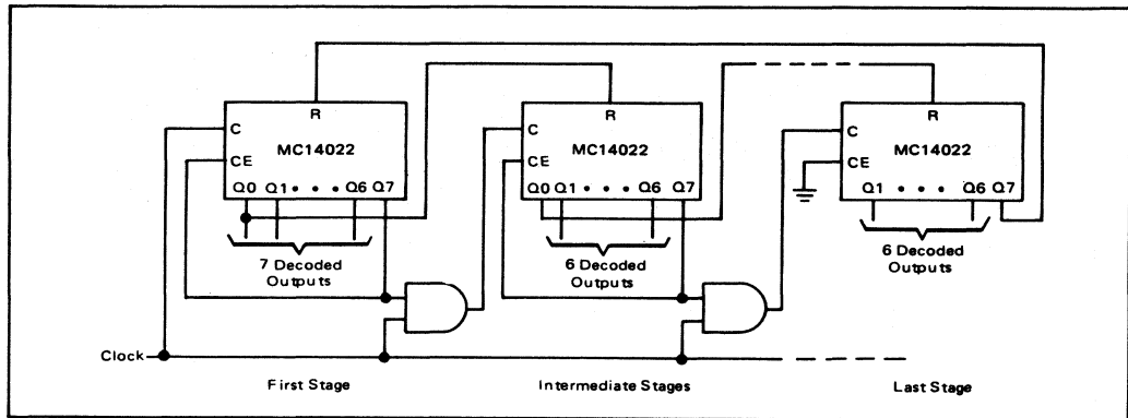
FIGURE 4 – COUNTER EXPANSION
