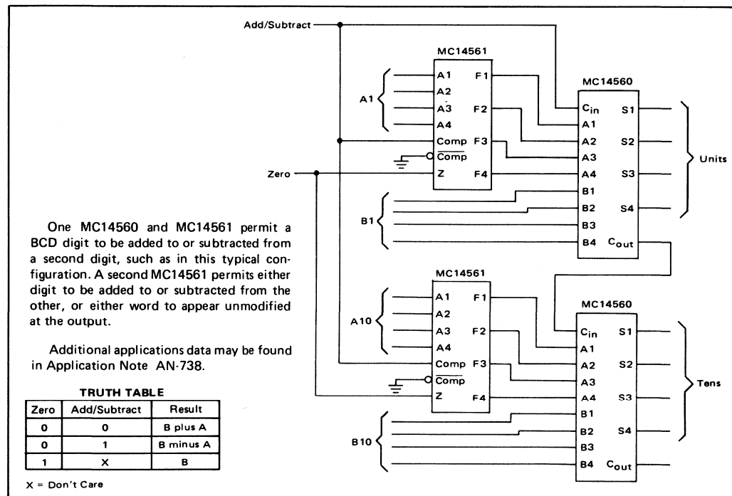
FIGURE 3 – PARALLEL ADD/SUBTRACT CIRCUIT
