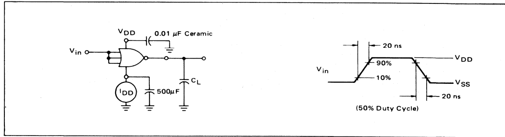
FIGURE 7 – SWITCHING TIME TEST CIRCUIT AND WAVEFORMS
