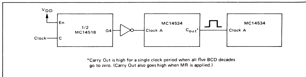
FIGURE 1 – CASCADE OPERATION
