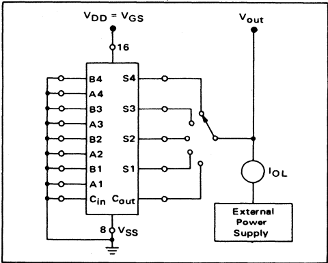
FIGURE 2 – TYPICAL SINK CURRENT CHARACTERISTICS TEST CIRCUIT
