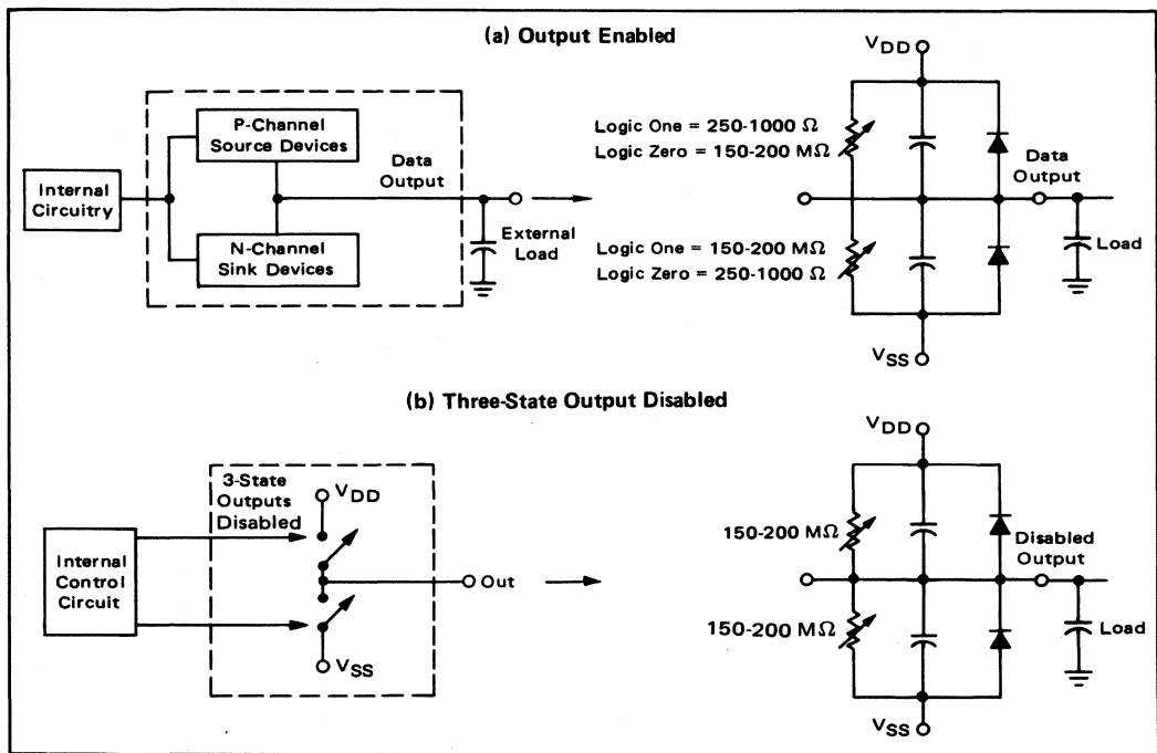
FIGURE 2-32 – CMOS OUTPUT EQUIVALENTS
