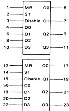
MC14508 Dual 4-Bit Latch
