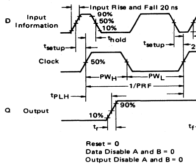
FIGURE 1 – TIMING DIAGRAM
