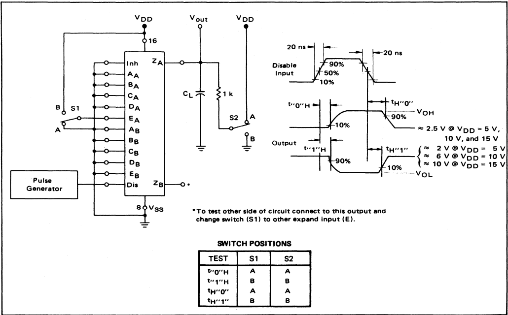
FIGURE 7 – SWITCHING TIME TEST CIRCUIT AND WAVEFORMS (For 3-State Output)
