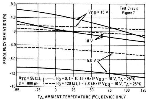
FIGURE 5 – RC OSCILLATOR STABILITY
