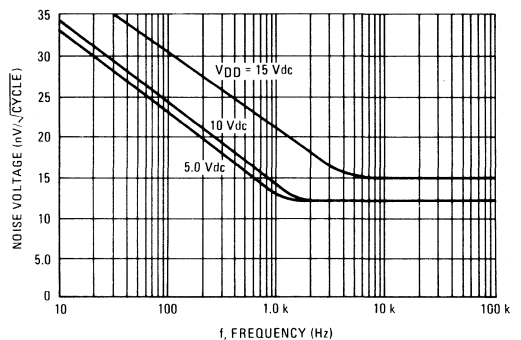
FIGURE 12 – TYPICAL NOISE CHARACTERISTICS
