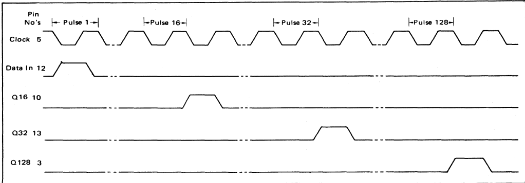
TIMING DIAGRAM
