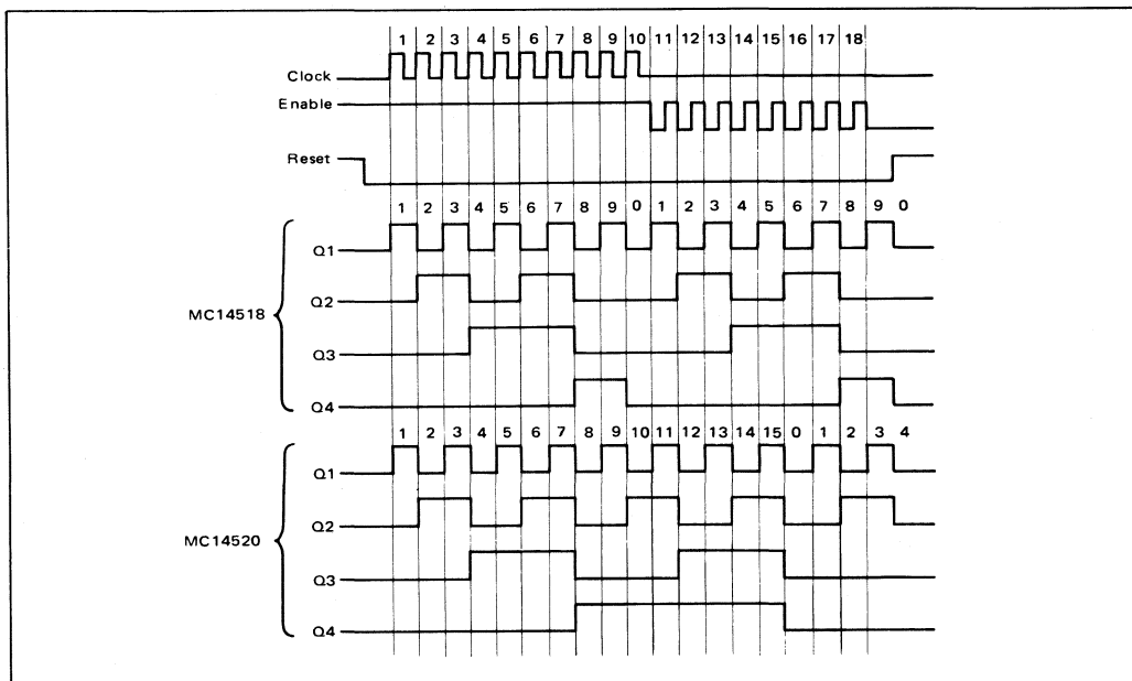
FIGURE 3 – TIMING DIAGRAM
