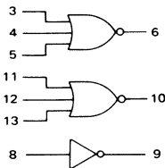
MC14000 Dual 3-Input NOR Gate plus Inverter
