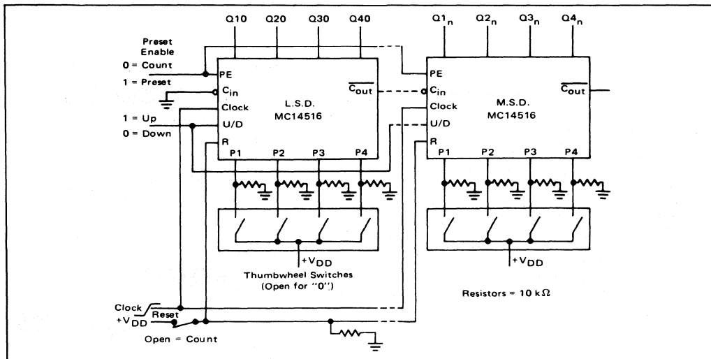
FIGURE 4 – PROGRAMMABLE CASCADED FREQUENCY DIVIDER
