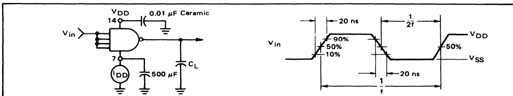
FIGURE 3 – POWER DISSIPATION TEST CIRCUIT AND WAVEFORM
