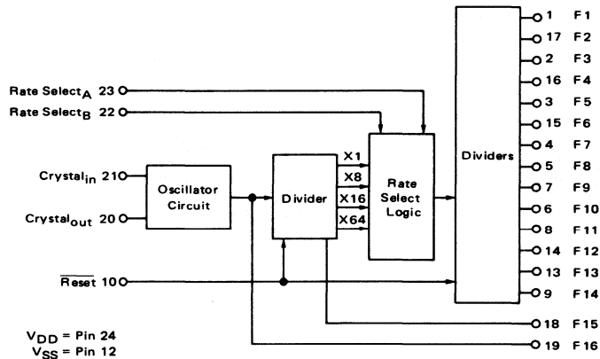
MC14411 Bit Rate Generator
