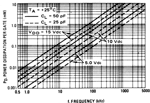
FIGURE 3 – GATE POWER DISSIPATION CHARACTERISTICS
