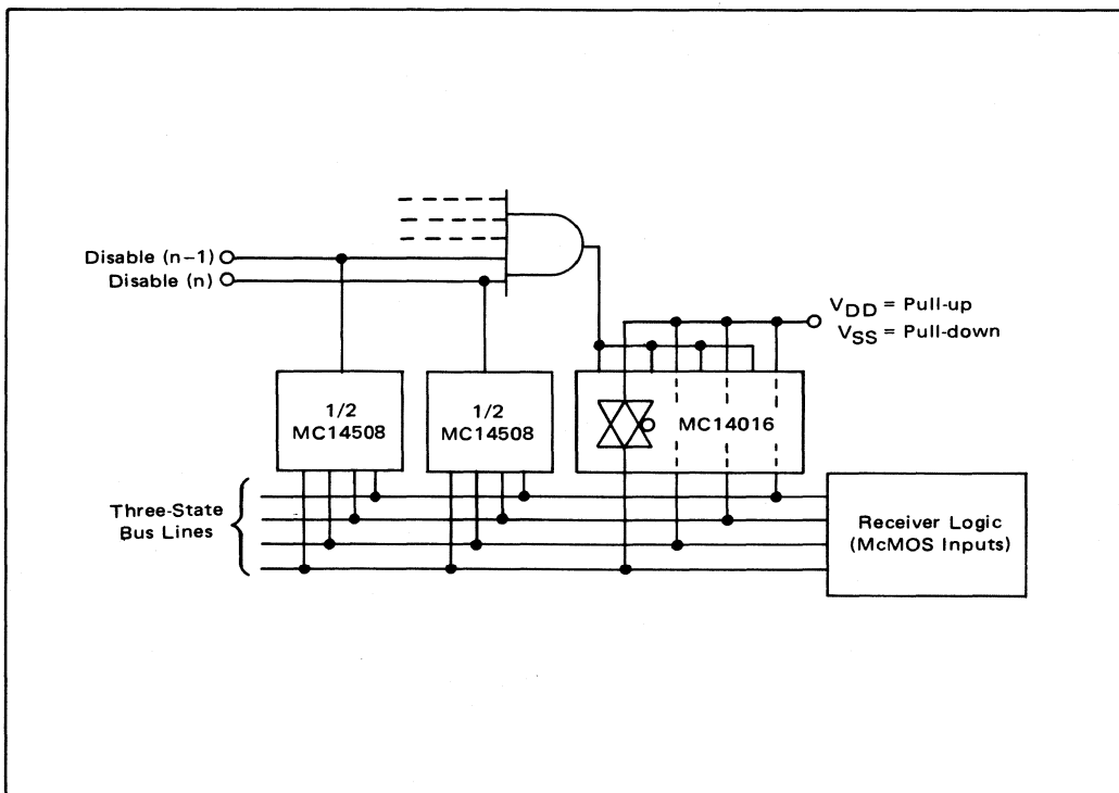
FIGURE 2-40 — THREE-STATE BUSING USING ACTIVE PULL-UP/PULL-DOWN
