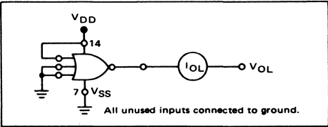
FIGURE 5 – TYPICAL OUTPUT SINK CHARACTERISTICS TEST CIRCUIT
