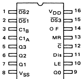
MC14553 3-Digit BCD Counter
