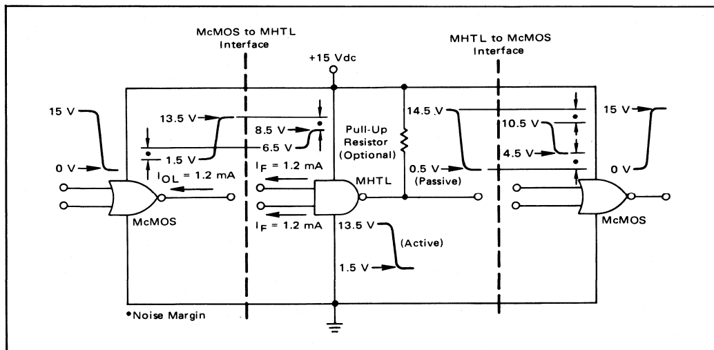
FIGURE 2-21 – INTERFACING CONDITIONS BETWEEN CMOS AND MHTL CIRCUITS
