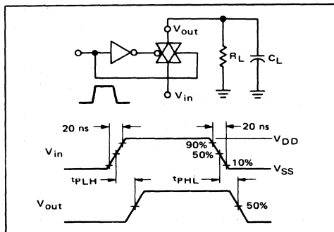
FIGURE 8 – PROPAGATION DELAY TEST CIRCUIT AND WAVEFORMS
