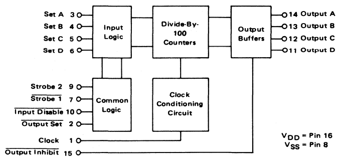
MC14415 Quad Precision Timer/Driver
