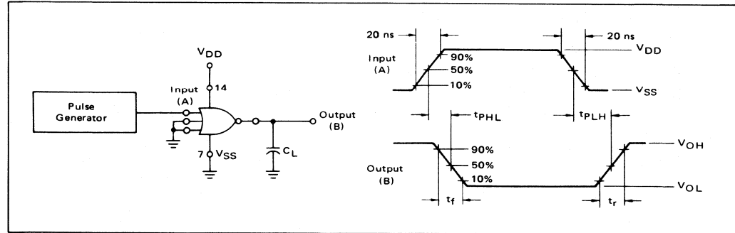
FIGURE 7 – SWITCHING TIME TEST CIRCUIT AND WAVEFORMS
