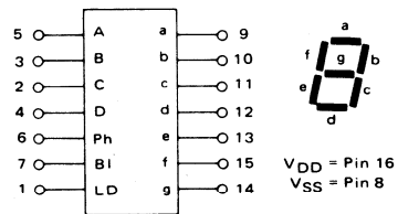
MC14543 BCD-To-Seven Segment Latch/Decoder/Driver
