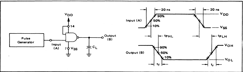
FIGURE 4 – SWITCHING TIME TEST CIRCUIT AND WAVEFORMS
