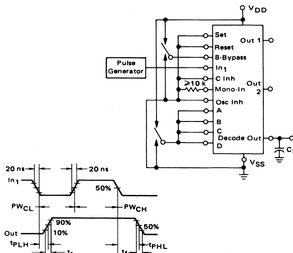
FIGURE 10 – SWITCHING TIME TEST CIRCUIT AND WAVEFORMS
