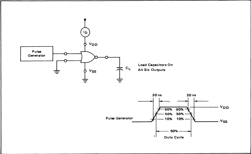
FIGURE 2 – POWER DISSIPATION TEST CIRCUIT AND WAVEFORM
