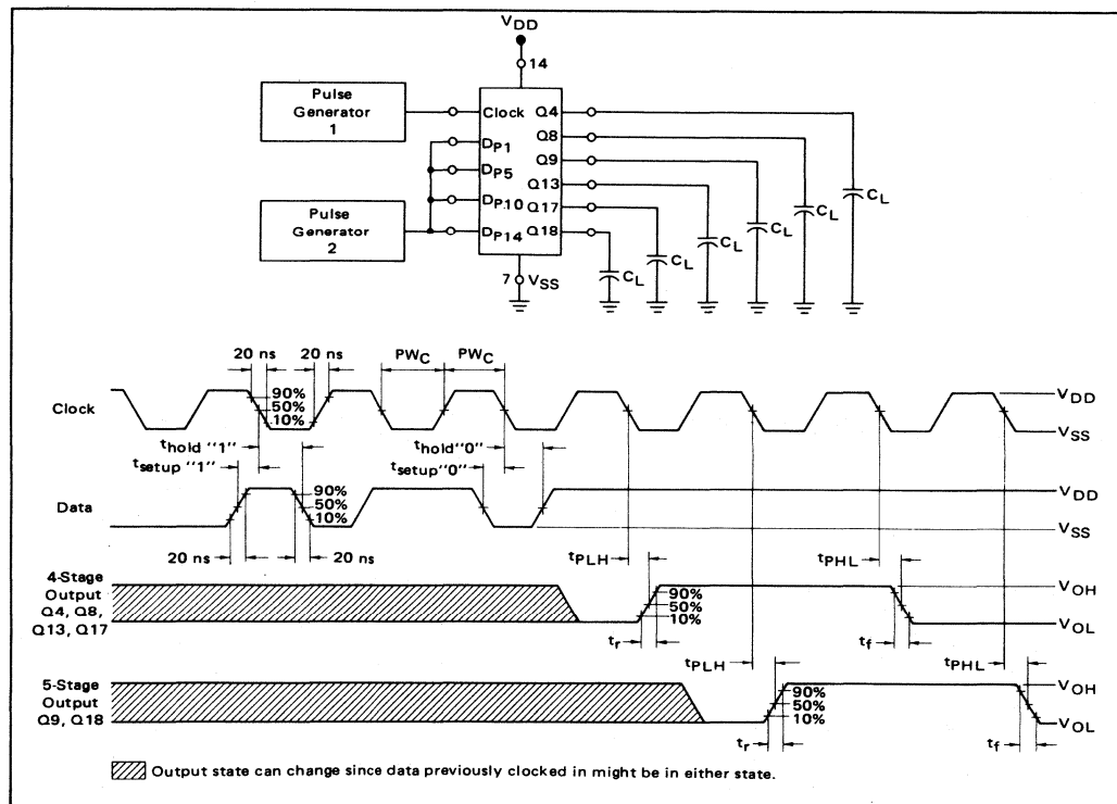
FIGURE 4 – SWITCHING TIME TEST CIRCUIT AND WAVEFORMS
