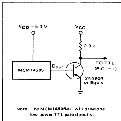
FIGURE 11 – CMOS-TO-TTL INTERFACE FOR V_{DD} = 5.0\text{ V}
