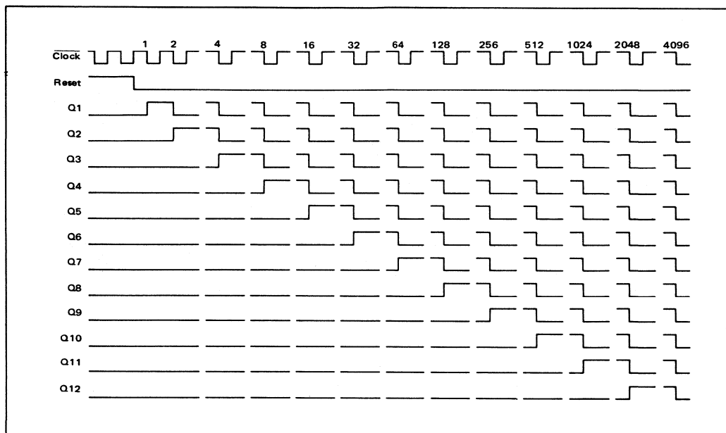
FIGURE 3 – TIMING DIAGRAM
