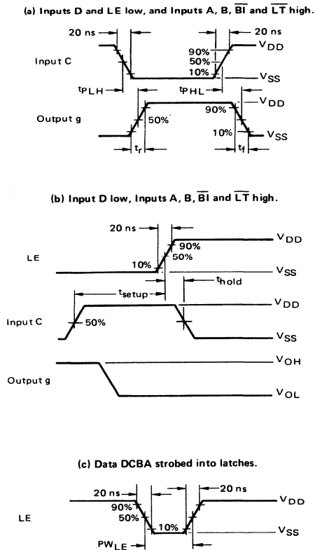
FIGURE 2 – DYNAMIC SIGNAL WAVEFORMS
