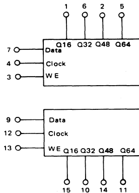
MC14562 128-Bit Static Shift Register
