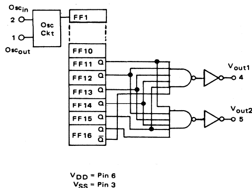
MC14450 Oscillator/2 16 Divider/Buffer
