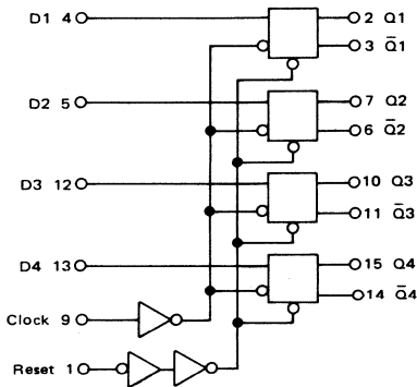
MC14175 Quad Type D Flip-Flop
