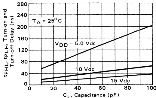
FIGURE 2-30 — TYPICAL PROPAGATION DELAY TIMES versus LOAD CAPACITANCE
