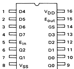
MC14532 8-Bit Priority Encoder
