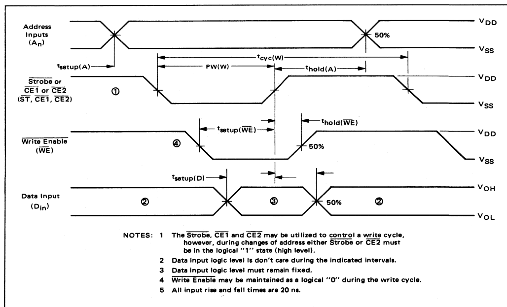
FIGURE 7 – WRITE CYCLE WAVEFORMS
