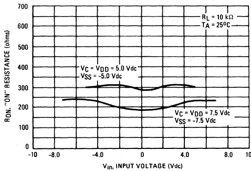
FIGURE 6 – V_{SS} = -5.0 V and -7.5 V
