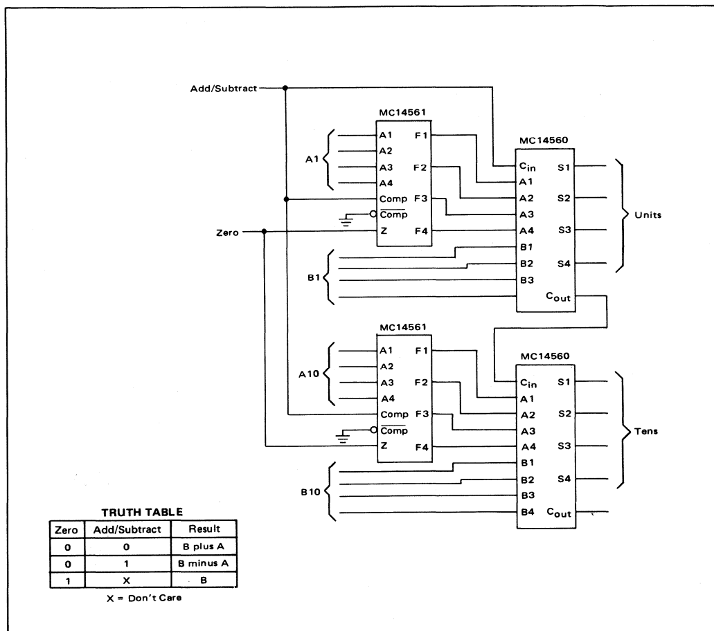
FIGURE 2 – PARALLEL ADD/SUBTRACT CIRCUIT (10's COMPLEMENT)
