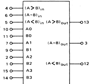
MC14585 4-Bit Magnitude Comparator
