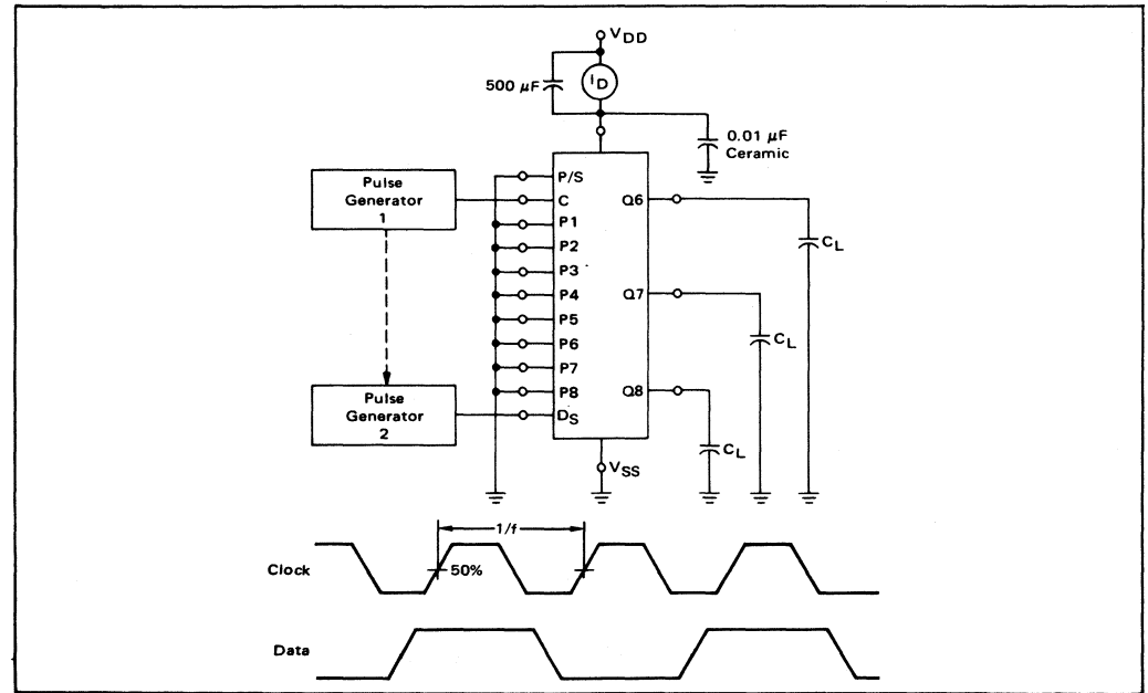
FIGURE 1 – POWER DISSIPATION TEST CIRCUIT AND WAVEFORM
