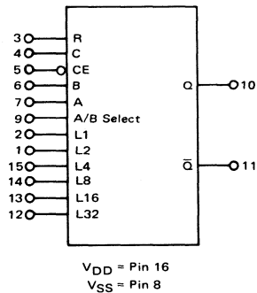
MC14557 1 to 64 Bit Variable Length Shift Register
