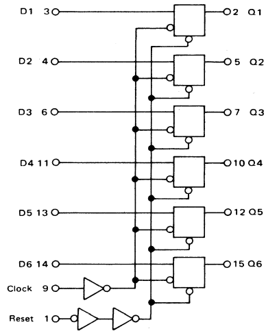
MC14174 Hex Type D Flip-Flop
