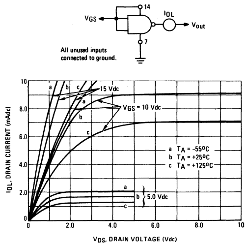
FIGURE 2 – TYPICAL OUTPUT SINK CHARACTERISTICS TEST CIRCUIT
