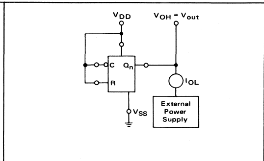
FIGURE 2 — TYPICAL OUTPUT SINK CHARACTERISTICS TEST CIRCUIT
