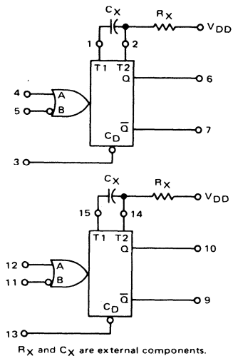
MC14528 Dual Retriggerable/Resetttable Monostable Multivibrator
