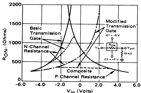
FIGURE 2-36 – McMOS TRANSMISSION GATES R_{ON} versus V_{in}
