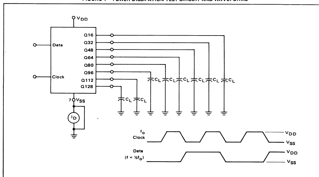
FIGURE 1 — POWER DISSIPATION TEST CIRCUIT AND WAVEFORMS
