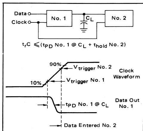
FIGURE 2-16 – SYNCHRONOUS OPERATION LIMITED BY CLOCK TRANSITION TIME
