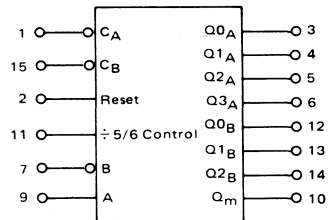
MC14566 Industrial Time Base Generator
