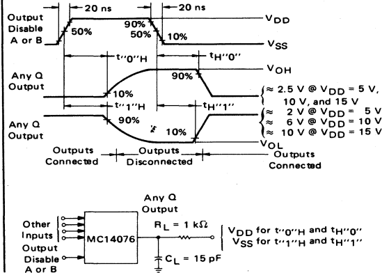
FIGURE 2 – THREE-STATE PROPAGATION DELAY WAVESHAPES AND CIRCUIT
