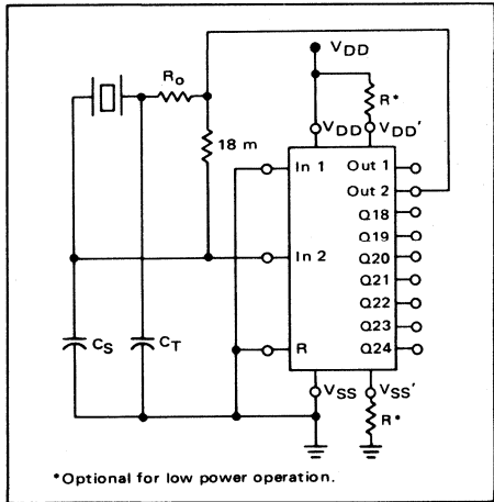
FIGURE 3 – CRYSTAL OSCILLATOR CIRCUIT
