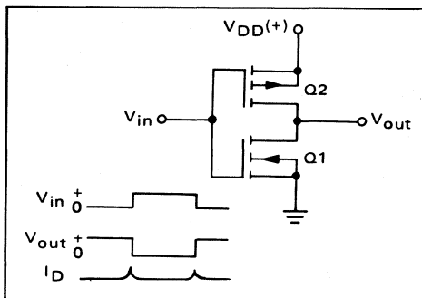
FIGURE 1-4 – TYPICAL COMPLEMENTARY INVERTER
