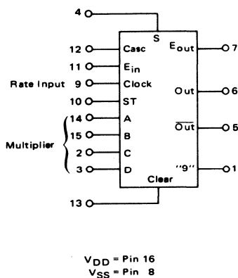
MC14527 BCD Rate Multiplier
