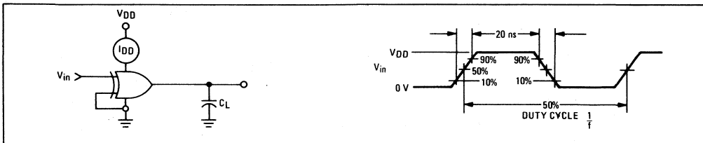
FIGURE 4 – POWER DISSIPATION TEST CIRCUIT AND WAVEFORM
