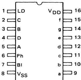
MC14543 BCD-To-Seven Segment Latch/ Decoder/Driver
