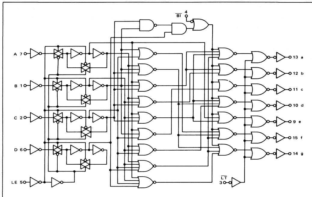
LOGIC DIAGRAM
