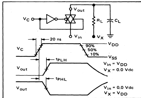
FIGURE 9 – TURN-ON DELAY TEST CIRCUIT AND WAVEFORMS
