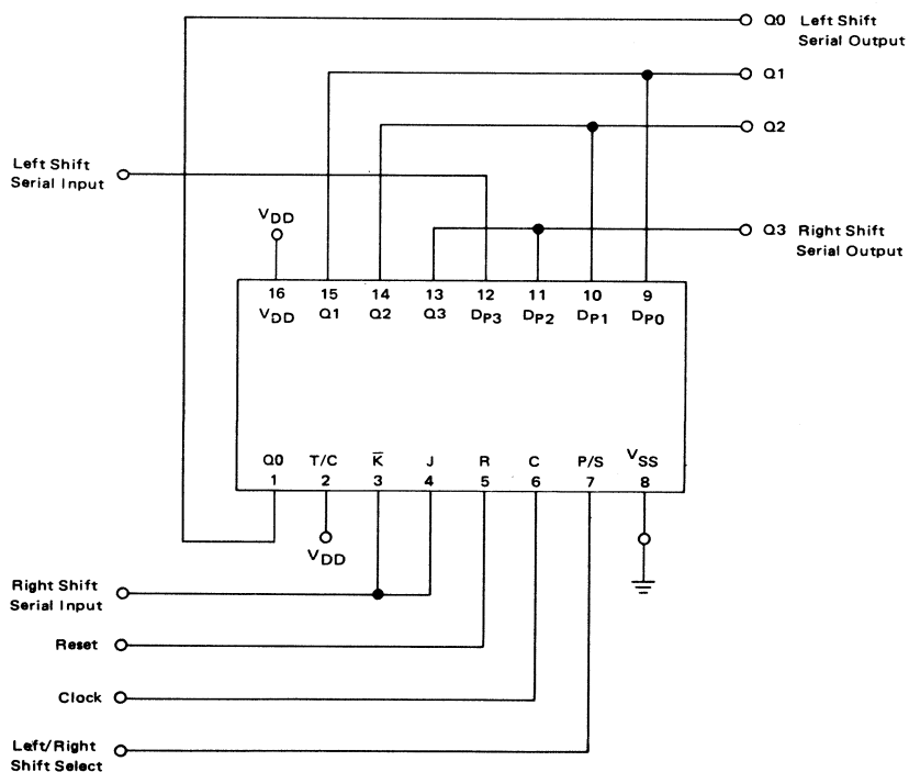
APPLICATION DIAGRAM Shift Left/Shift Right Register
