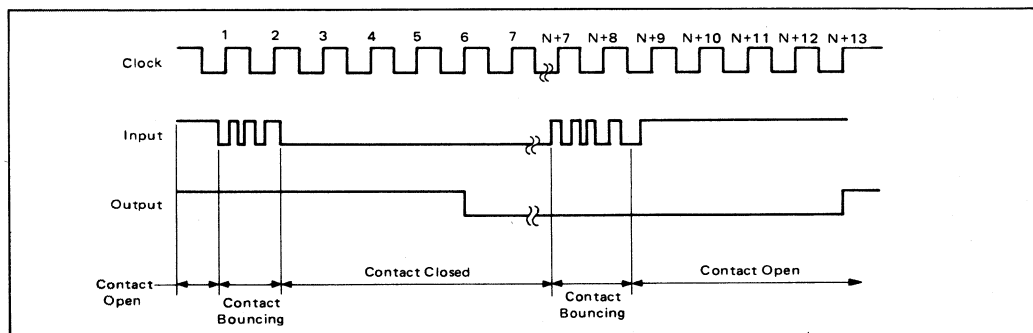
FIGURE 3 — TIMING DIAGRAM
