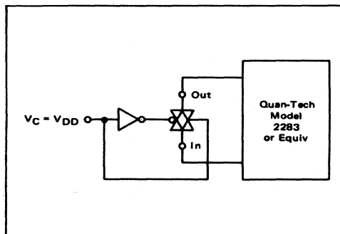
FIGURE 15 – NOISE VOLTAGE TEST CIRCUIT
