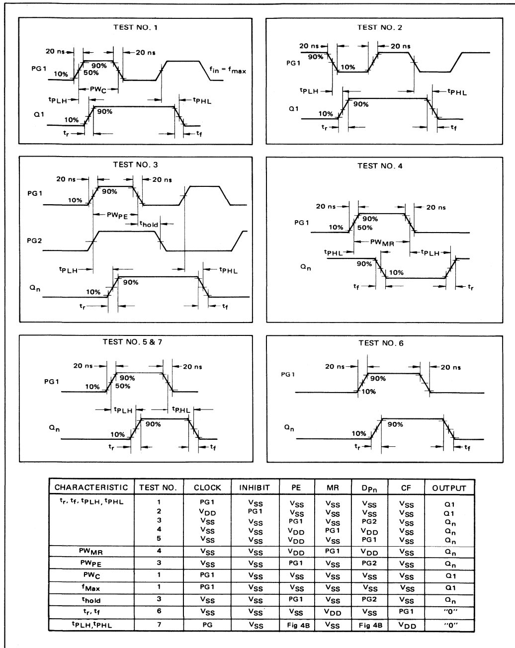
FIGURE 5 – AC TEST CONNECTIONS AND WAVEFORMS
