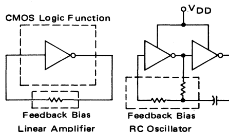
FIGURE 2-2 — LINEAR BIASING SCHEMES
