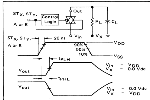
FIGURE 8 – TURN-ON DELAY TIME TEST CIRCUIT AND WAVEFORMS
