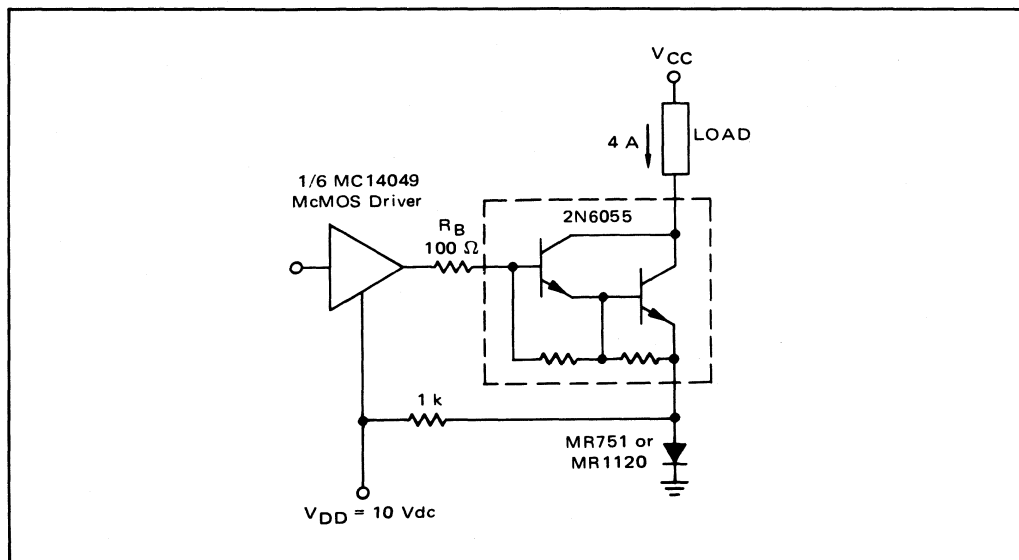
FIGURE 2-28 – CMOS TO BIPOLAR 4 AMPERE DRIVER
