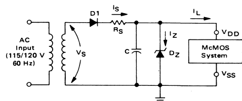
FIGURE 2-8(a) – CMOS UNREGULATED POWER SUPPLY
