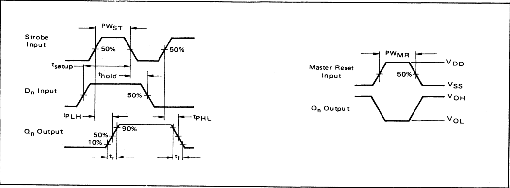
FIGURE 1 – AC WAVEFORMS
