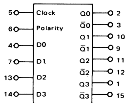
MC14042 Quad Latch
