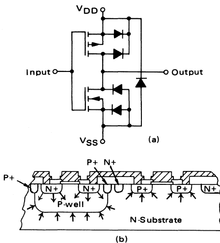
FIGURE 2-3 – LEAKAGE CURRENTS OF P-N DIODE JUNCTIONS
