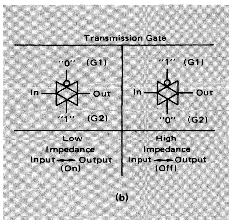
FIGURE 2-34 – BASIC THREE-STATE OUTPUTS
