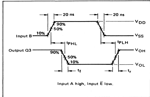
FIGURE 3 – DYNAMIC SIGNAL WAVEFORMS (MC14556)
