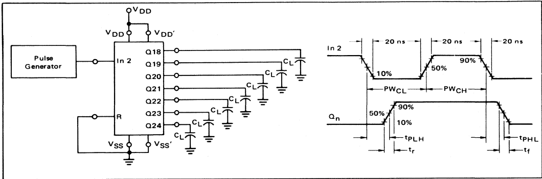
FIGURE 2 – SWITCHING TIME TEST CIRCUIT AND WAVEFORMS
