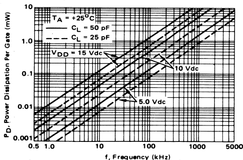
FIGURE 2-6 – TYPICAL GATE POWER DISSIPATION CHARACTERISTICS
