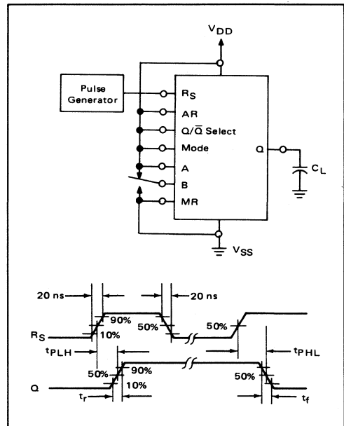
FIGURE 2 – SWITCHING TIME TEST CIRCUIT AND WAVEFORMS
