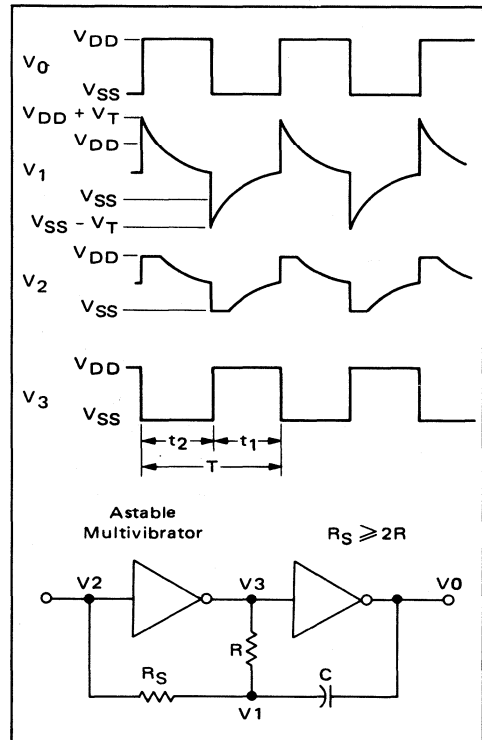
FIGURE 2-15 – ASTABLE MULTIVIBRATOR WITH ADDITION OF COMPENSATING RESISTOR R_S
