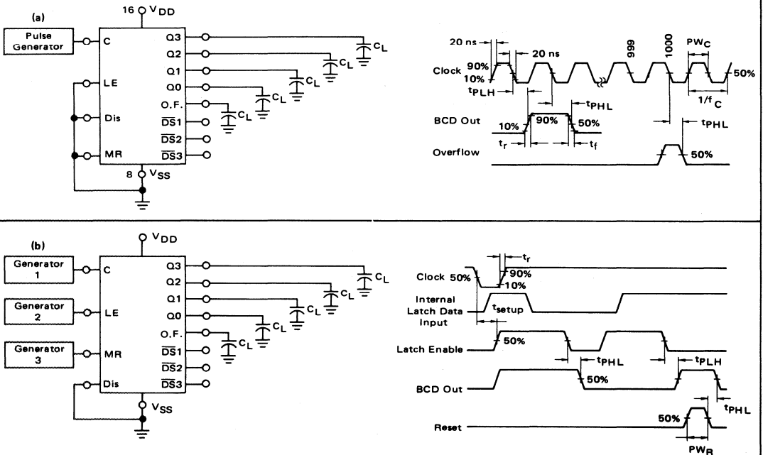
FIGURE 3 – SWITCHING TIME TEST CIRCUITS AND WAVEFORMS
