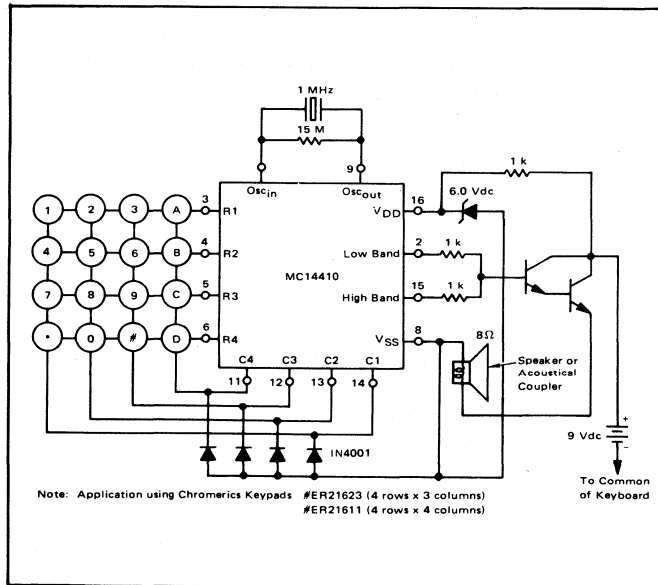
FIGURE 6 – BATTERY POWERED OPERATION (Driving Audio Speaker)
