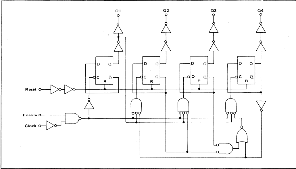
FIGURE 4 – DECADE COUNTER (MC14518) LOGIC DIAGRAM (1/2 OF DEVICE SHOWN)
