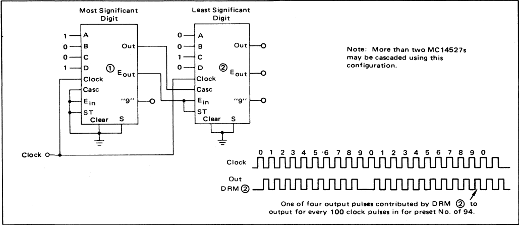
FIGURE 4 — TWO MC14527s IN CASCADE WITH PRESET NO. OF 94
