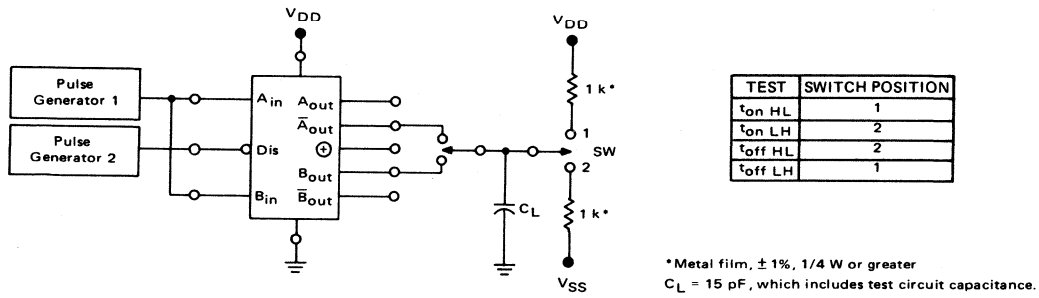
FIGURE 5 – 3-STATE SWITCHING TIME TEST CIRCUIT AND WAVEFORMS
