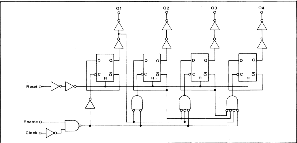
FIGURE 5 – BINARY COUNTER (MC14520) LOGIC DIAGRAM (1/2 OF DEVICE SHOWN)
