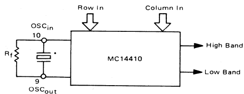
FIGURE 3 – TYPICAL CRYSTAL CIRCUIT
