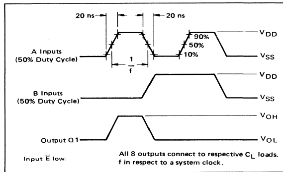
FIGURE 1 – DYNAMIC POWER DISSIPATION SIGNAL WAVEFORMS
