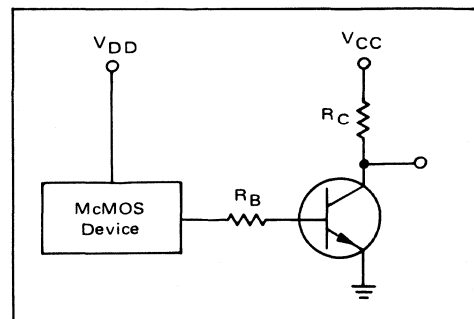
FIGURE 2-27 – McMos to Discrete Interface
