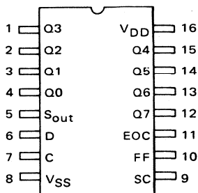
MC14559 Successive Approximation Register
