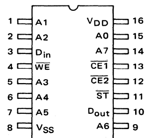
MC14537 256-Bit Static Random Access Memory
