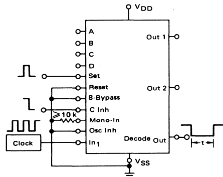
FIGURE 1 – TIME INTERVAL CONFIGURATION USING EXTERNAL CLOCK; SET AND CLOCK INHIBIT FUNCTIONS
