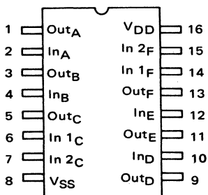
MC14572 Hex Gate
