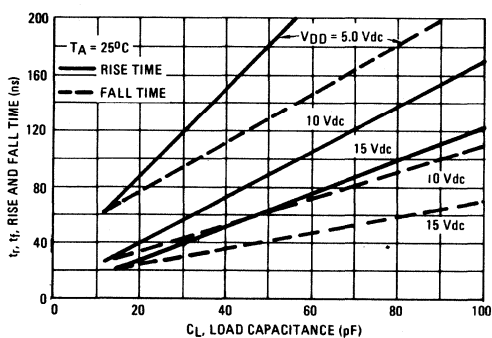
FIGURE 4 – RISE AND FALL TIME versus LOAD CAPACITANCE
