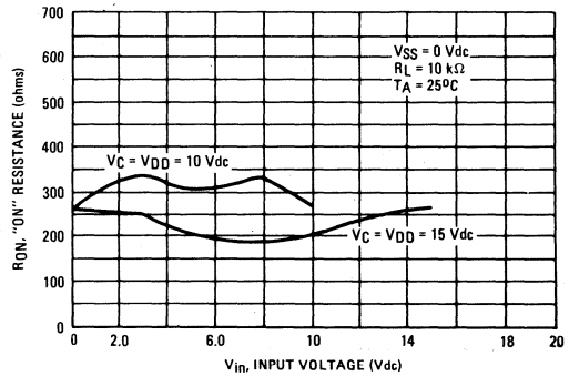
FIGURE 7 – V_{SS} = 0 V
