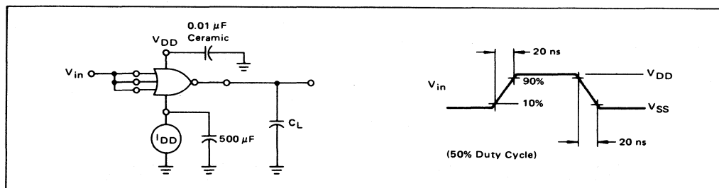
FIGURE 7 – POWER DISSIPATION TEST CIRCUIT AND WAVEFORM
