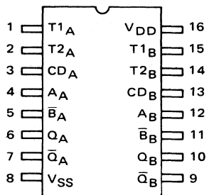
MC14528 Dual Retriggerable/Resettable Monostable Multivibrator
