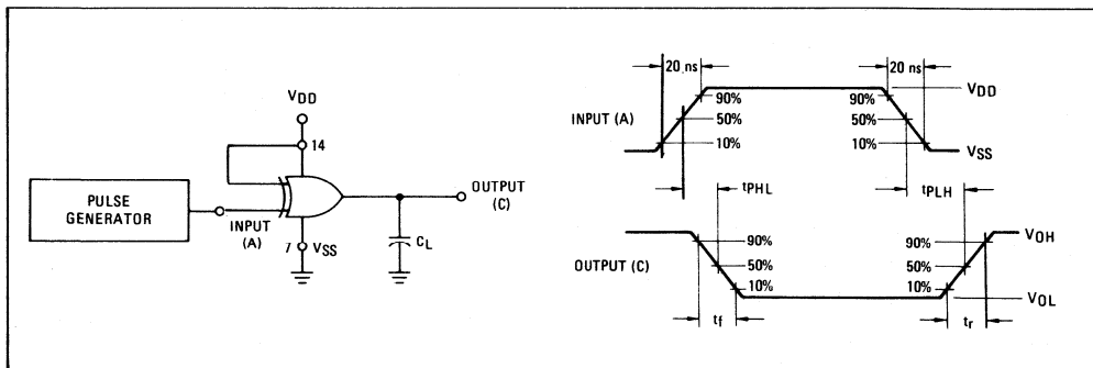
FIGURE 5 – SWITCHING TIME TEST CIRCUIT AND WAVEFORMS
