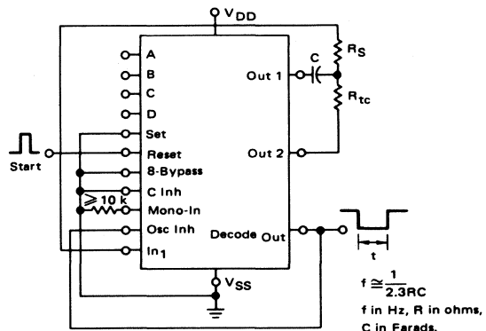
FIGURE 3 – TIME INTERVAL CONFIGURATION USING ON-CHIP RC OSCILLATOR AND RESET INPUT TO INITIATE TIME INTERVAL
