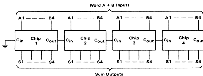
FIGURE 6 – USING THE MC14008 IN A 16-BIT ADDER CONFIGURATION
