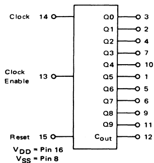
MC14017 Decade Counter/Divider
