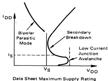
FIGURE 2-1 — SECONDARY BREAKDOWN CHARACTERISTICS
