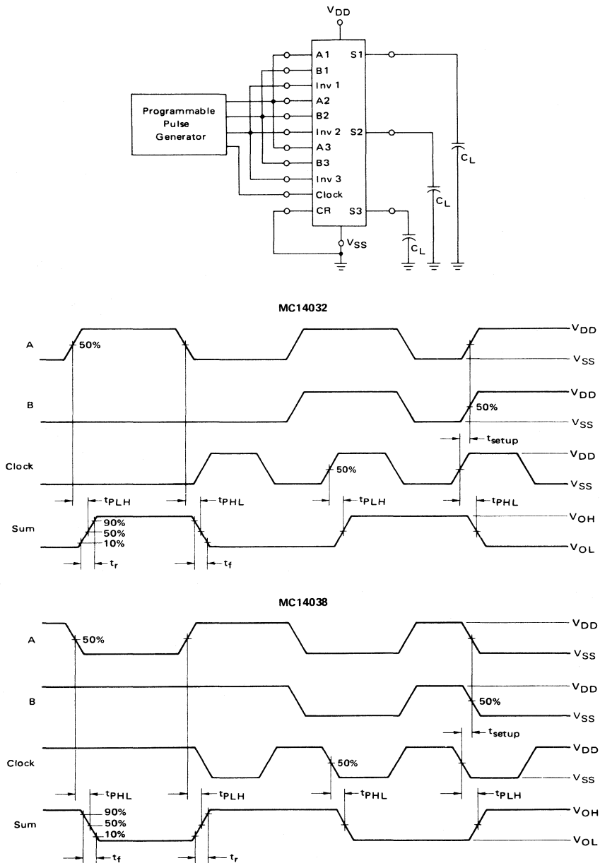
FIGURE 4 – SWITCHING TIME TEST CIRCUIT AND WAVEFORMS
