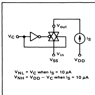
FIGURE 2 – NOISE IMMUNITY TEST CIRCUIT
