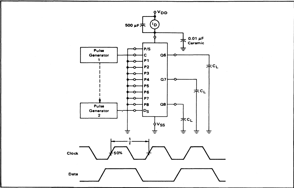
FIGURE 3 – POWER DISSIPATION TEST CIRCUIT AND WAVEFORM
