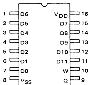
MC14531 12-Bit Parity Tree
