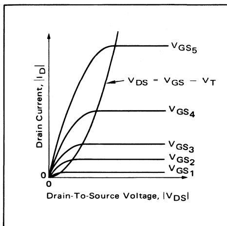
FIGURE 2-17 – OUTPUT DRAIN CHARACTERISTICS
