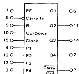
MC14510 - BCD MC14516 - Binary } Up/Down Counters
