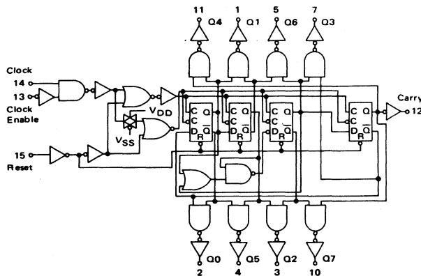
LOGIC DIAGRAM
