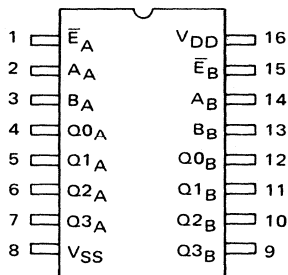
MC14555 Dual Binary to 1-of-4 Decoder/ Demultiplexer
