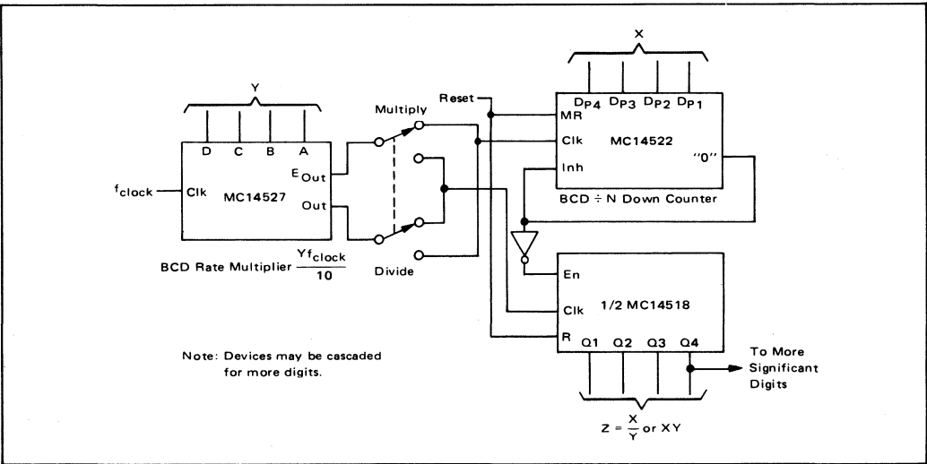
FIGURE 5 — MULTIPLIER/DIVIDER APPLICATION
