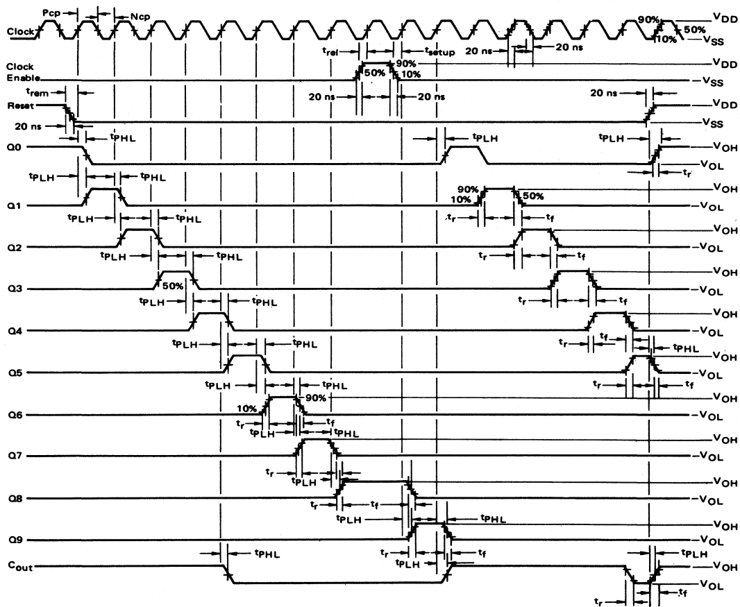
FIGURE 3 – AC MEASUREMENT DEFINITION AND FUNCTIONAL WAVEFORMS
