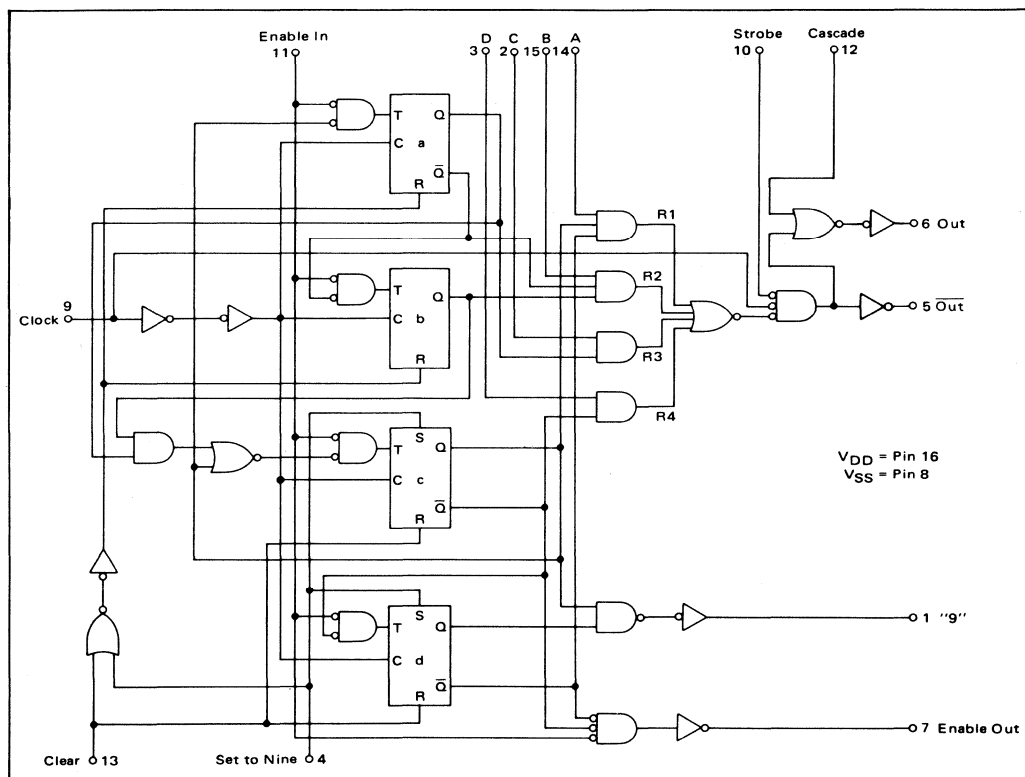
LOGIC DIAGRAM
