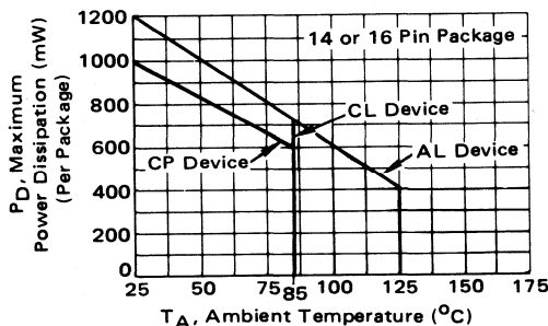
FIGURE 2-10 – AMBIENT TEMPERATURE POWER DERATING
