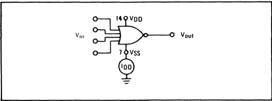
FIGURE 1 – CURRENT AND VOLTAGE TRANSFER CHARACTERISTICS TEST CIRCUIT
