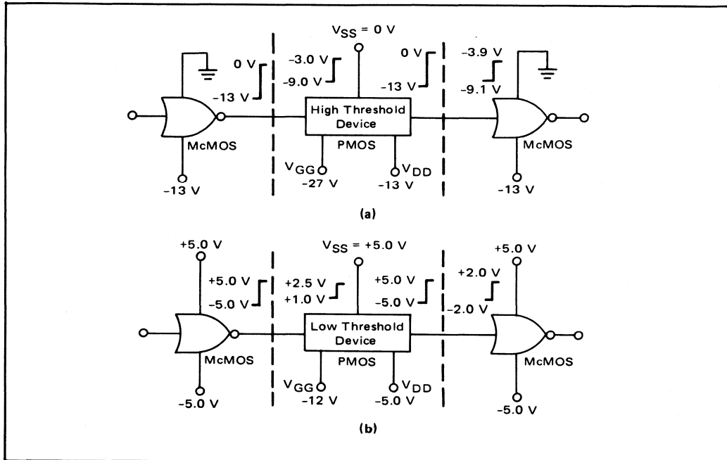
FIGURE 2-24 — McMOS — PMOS AND PMOS — McMOS INTERFACE SYSTEMS
