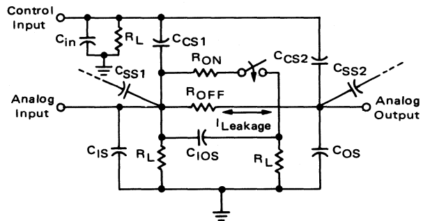
FIGURE 2-38 — AC MODEL OF SIMPLE TRANSMISSION GATE
