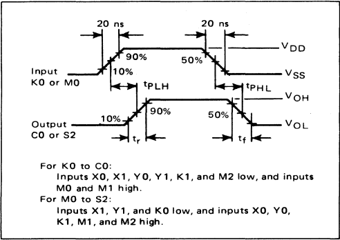
FIGURE 2 – DYNAMIC SIGNAL WAVEFORMS
