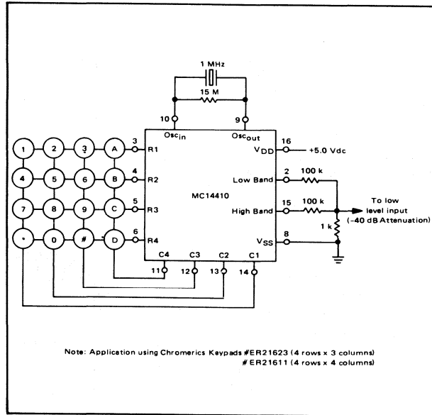
FIGURE 5 – LOW LEVEL OUTPUT TONE GENERATOR APPLICATION
