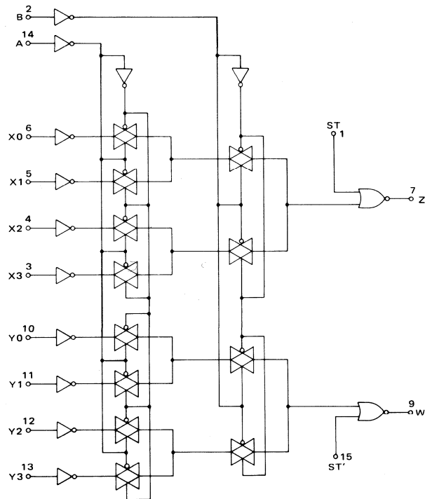
LOGIC DIAGRAM
