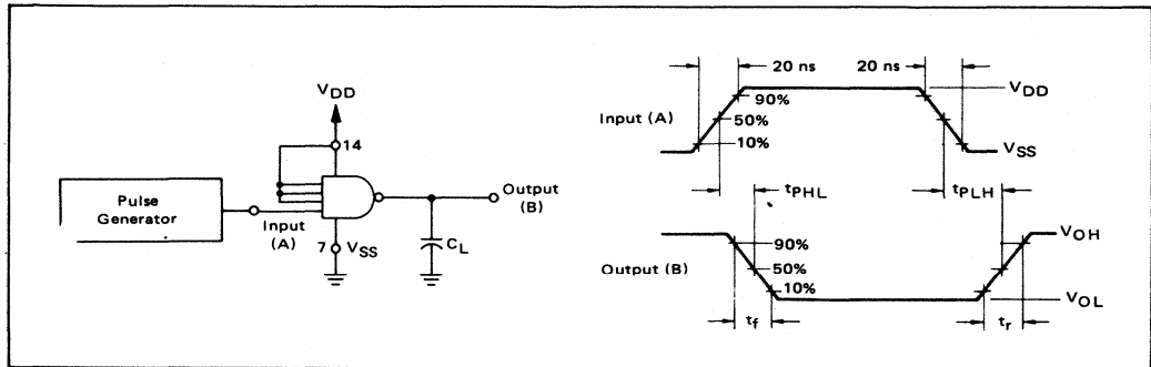
FIGURE 4 – SWITCHING TIME TEST CIRCUIT AND WAVEFORMS
