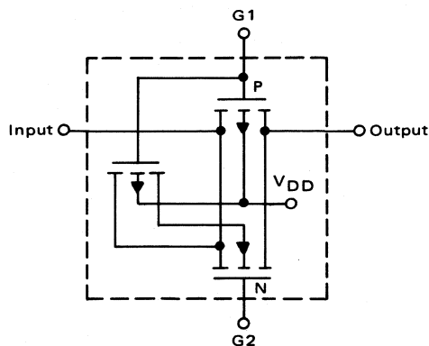
FIGURE 2-37 – MODIFIED McMOS TRANSMISSION GATE
