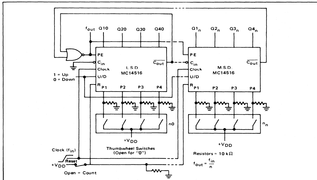
FIGURE 4 – PROGRAMMABLE CASCADED FREQUENCY DIVIDER
