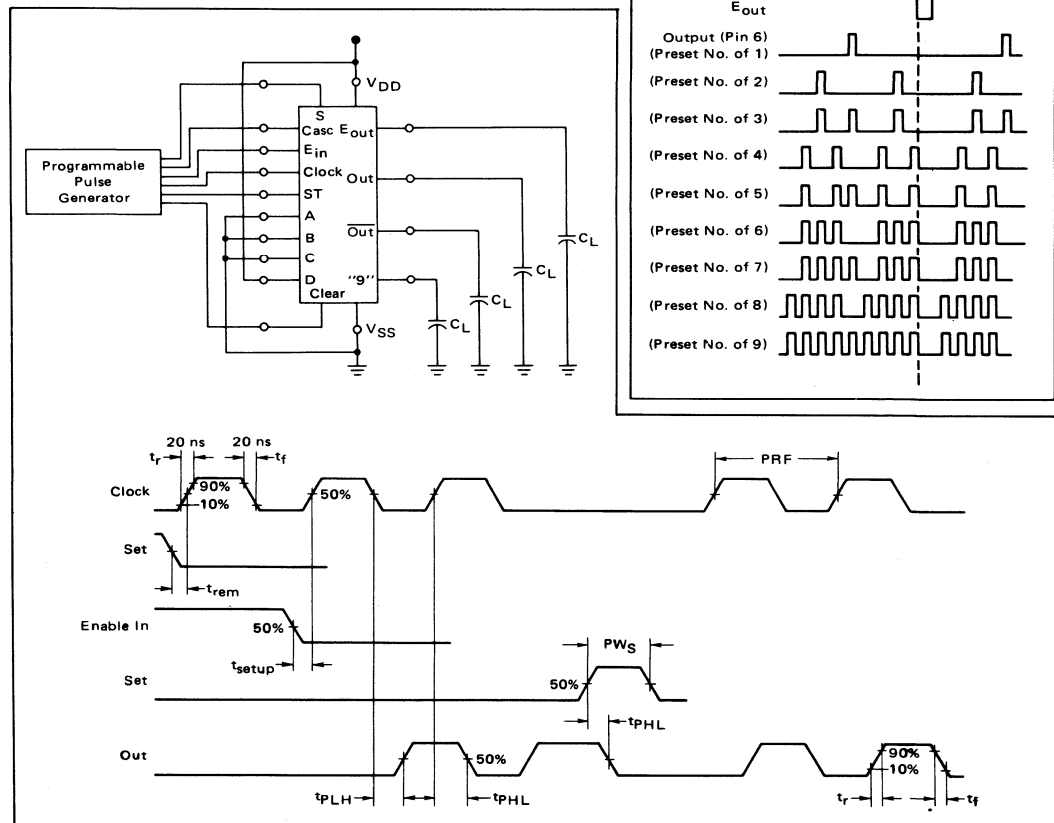
FIGURE 2 – SWITCHING TIME TEST CIRCUIT AND WAVEFORMS
