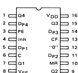
MC14522 Programmable Divide-By-N-4-Bit BCD Counter
