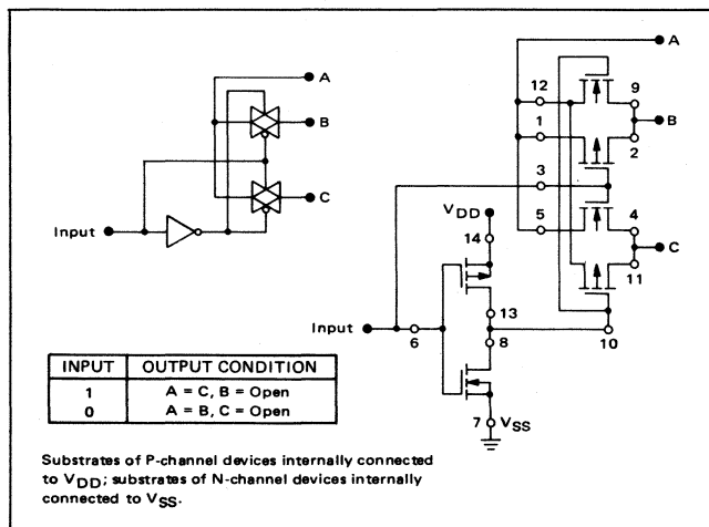
FIGURE 1 — TYPICAL APPLICATION: 2-INPUT ANALOG MULTIPLEXER
