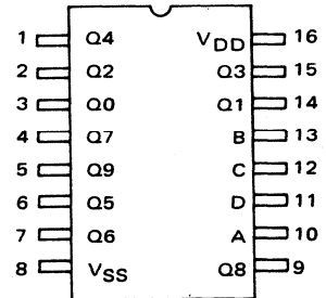
MC14028 BCD-To-Decimal Decoder/ Binary-To-Octal Decoder
