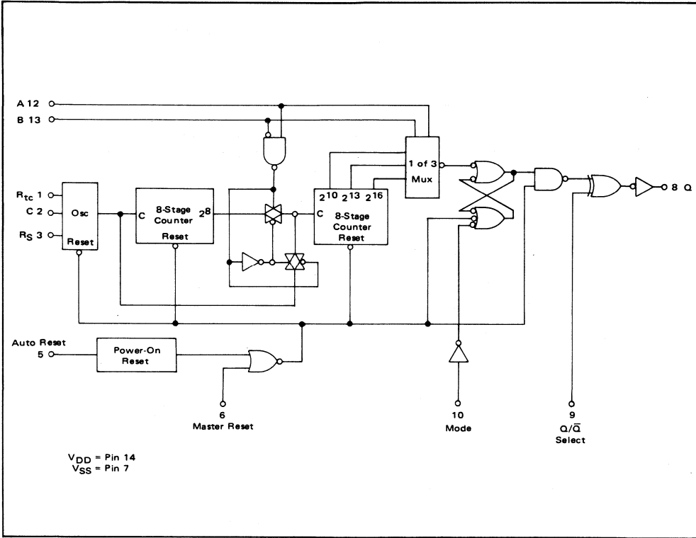
EXPANDED BLOCK DIAGRAM
