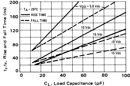
FIGURE 2-29 — TYPICAL RISE AND FALL TIME versus LOAD CAPACITANCE
