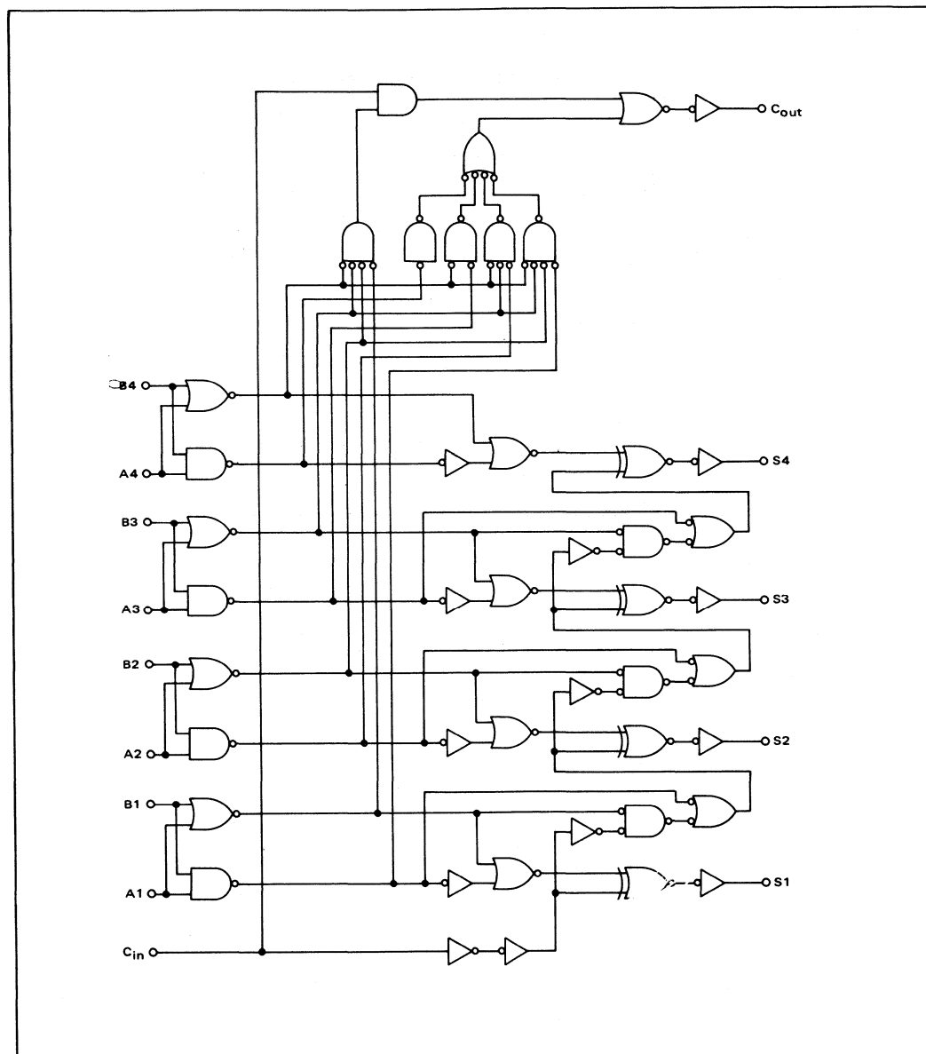
FIGURE 5 – LOGIC DIAGRAM
