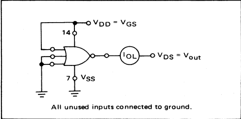
FIGURE 5 – TYPICAL SINK CURRENT CHARACTERISTICS TEST CIRCUIT
