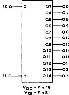
MC14020 14-Bit Binary Counter
