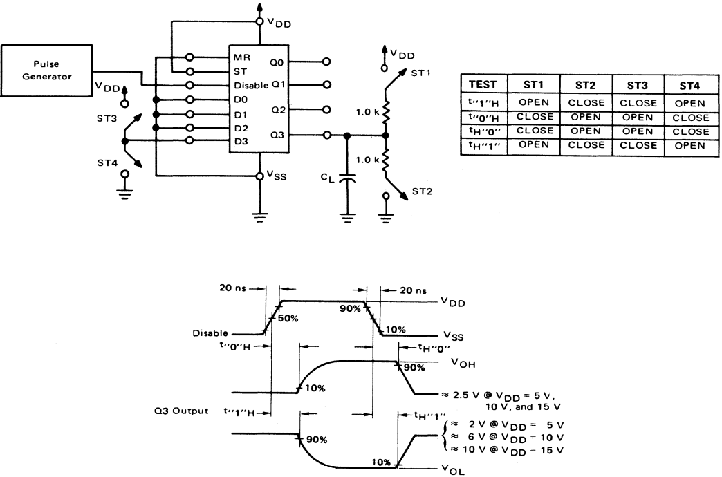
FIGURE 2 – 3-STATE AC TEST CIRCUIT AND WAVEFORMS
