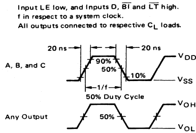
FIGURE 1 – DYNAMIC POWER DISSIPATION SIGNAL WAVEFORMS
