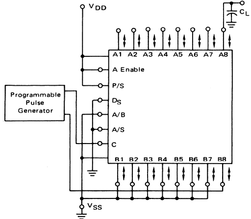
FIGURE 3 – B SYNCHRONOUS DATA INPUT, B PARALLEL DATA OUTPUT AND SETUP TIME
