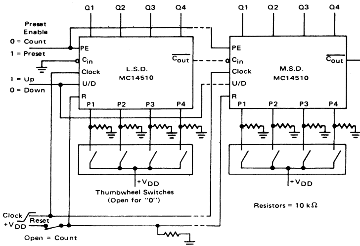
FIGURE 4 – PROGRAMMABLE CASCADED FREQUENCY DIVIDER
