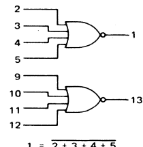
MC14002 Dual 4-Input NOR Gate
