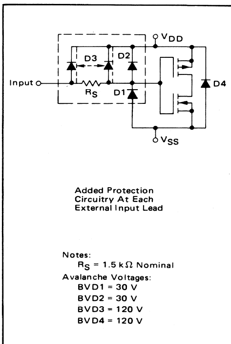
FIGURE 2-13(b) - SCHEMATIC DIAGRAM, DIODE-RESISTOR INPUT PROTECTION
