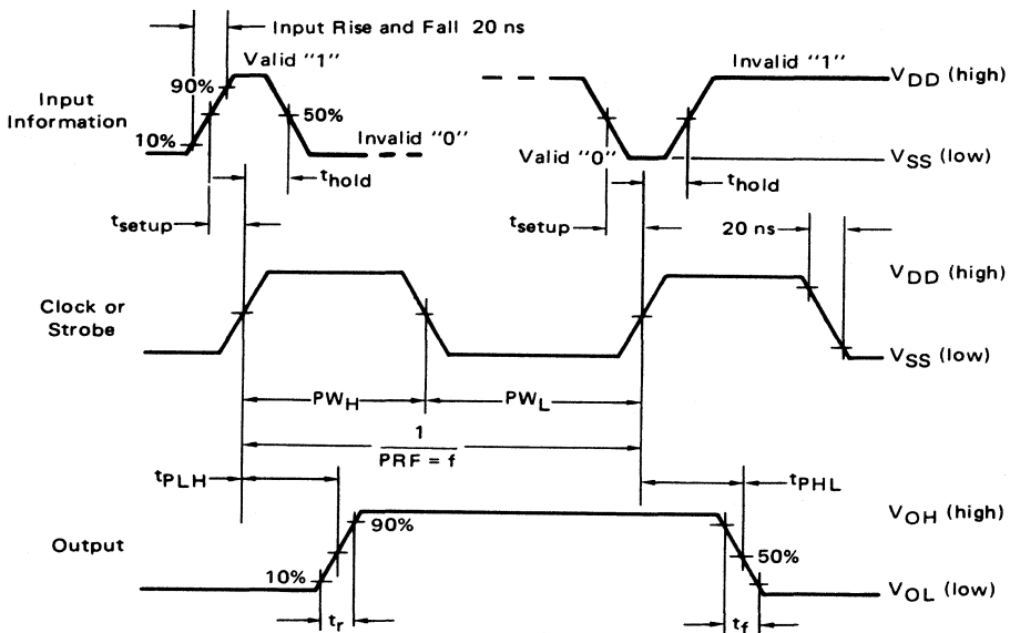
FIGURE 5-15 – SYNCHRONOUS CIRCUIT WAVESHAPES AND TIMING PARAMETERS
