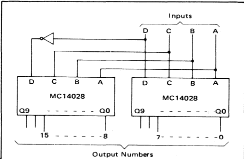
FIGURE 2 – CODE CONVERSION CIRCUIT AND TRUTH TABLE
