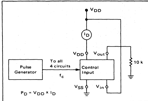
FIGURE 4 – QUIESCENT POWER DISSIPATION TEST CIRCUIT
