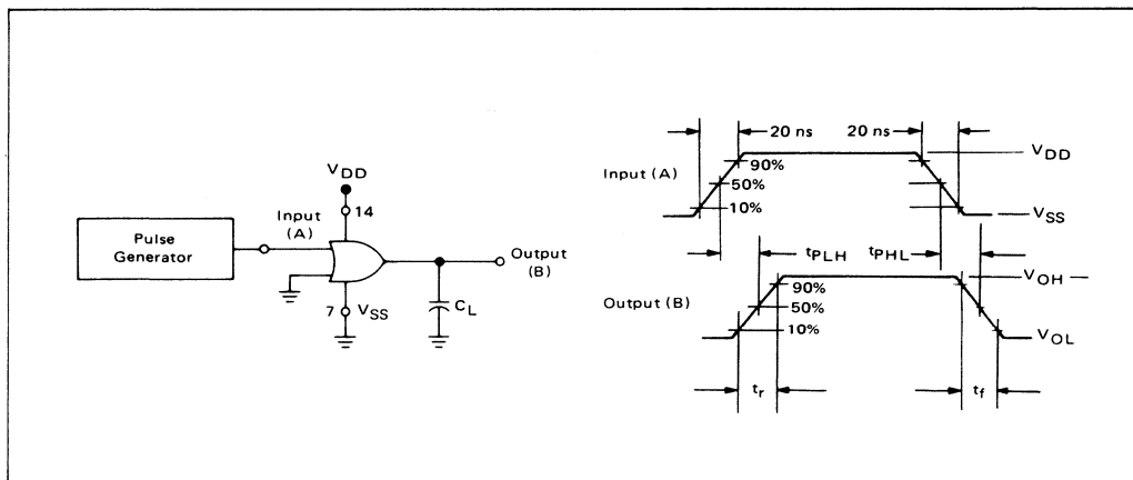
FIGURE 5 – SWITCHING TIME TEST CIRCUIT AND WAVEFORMS
