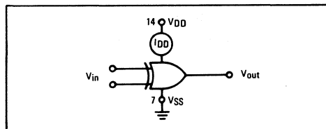
FIGURE 1 – CURRENT AND VOLTAGE TRANSFER CHARACTERISTICS TEST CIRCUIT
