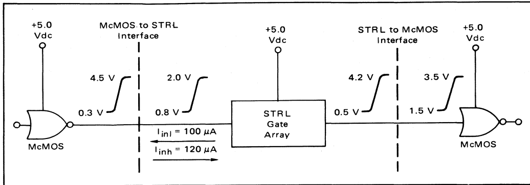
FIGURE 2-26 – McMos – STRL LSI SYSTEMS INTERFACE
