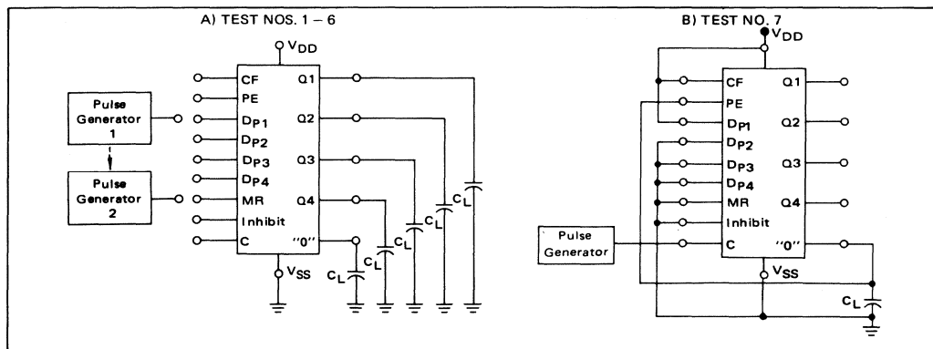
FIGURE 4 – AC TEST CIRCUITS
