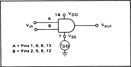
FIGURE 1 – CURRENT AND VOLTAGE TRANSFER CHARACTERISTICS TEST CIRCUIT
